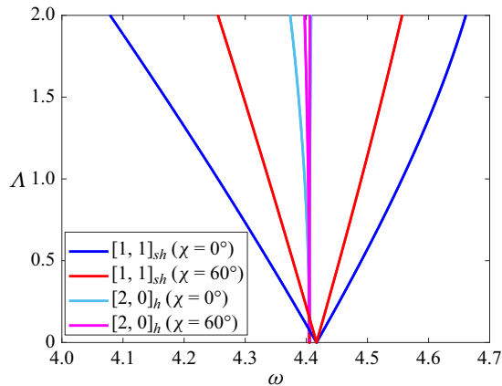
Figure 7. Instability tongues for [2, 0] harmonic and [1, 1] subharmonic modes plotted in the acceleration–frequency ( \Delta - \omega ) space, depending upon the slanting angle \chi = 0^\circ and 60^\circ , with pinned contact line and \alpha = 90^\circ .
