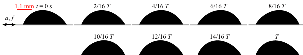
Figure 10. Harmonic rocking mode [1, 1] over a complete cycle of oscillation with period T , which has been excited at acceleration a = 0.25\text{ g} and frequency f = 63.5\text{ Hz} using horizontal \chi = 90^\circ vibration, with contact angle \alpha = 60.7^\circ and volume V = 4.6\text{ ml} .
