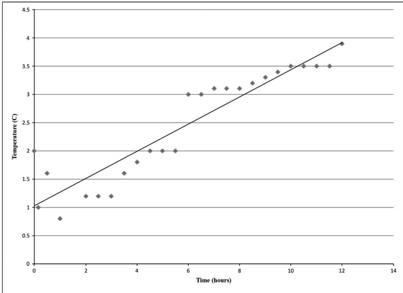
Figure 1. Saline Temperature over Time (Playmate Cooler)
