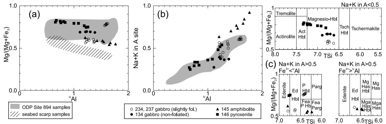
Figure 3. Amphibole compositions (expressed as atomic formula units on the basis of 23 oxygens) of the ophiolitic rocks of Ikaria, compared with amphiboles in oceanic crust at Hess Deep, from ODP Site 894 and samples from a seafloor scarp (from Manning, MacLeod & Weston, 2000). Nomenclature in panels (c) from Leake et al. (1997), abbreviations as follows: Act – actinolitic; Ed – edenitic; Fea – ferroan; Has – hastingsite, hastingsitic; Hb, Hbl – hornblende; Mg – magnesio; Mga – magnesian; P – pargasitic; Parg – pargasite; Tsch – tschermakitic.
