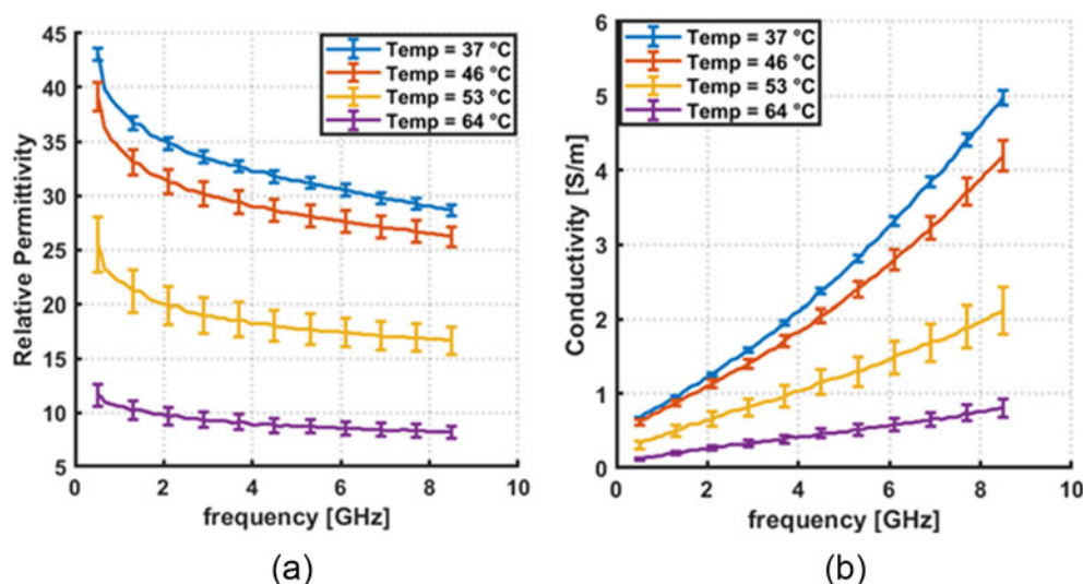
Figure 7. Temperature-dependent dielectric properties (a) relative permittivity and (b) conductivity for the adrenal medulla over 0.5–8.5 GHz frequency band. The temperature of the adrenal gland sample was raised to 37°C, 46°C, 53°C, and 64°C.
