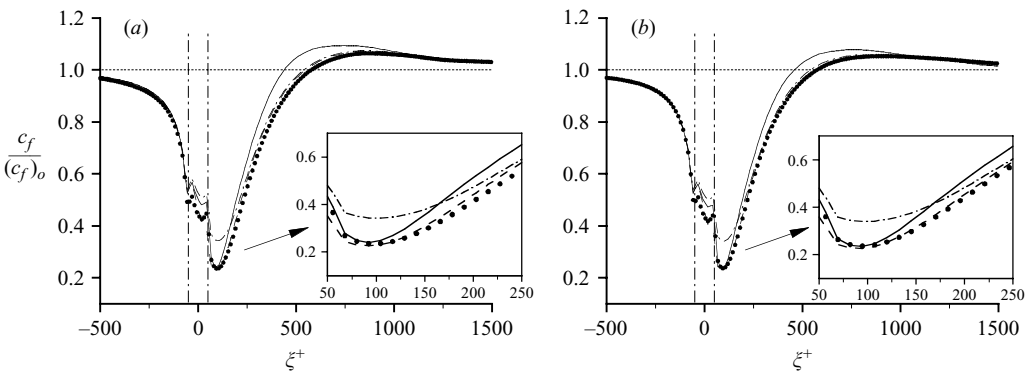
FIGURE 10. Variation of time-averaged skin friction in the streamwise direction due to periodic blowing: ---, f^+ = 0.010 ; —, f^+ = 0.035 ; ···, f^+ = 0.080 ; ●, SB ( f^+ = 0 ). (a) Re_\theta = 300 ; (b) 670.
