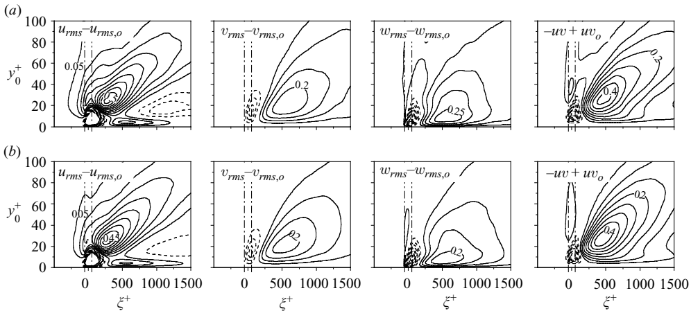
FIGURE 5. Contours of the difference between the time-averaged turbulent intensities and Reynolds shear stress for steady blowing and those for no blowing. Here, y_0^+ = y u_{\tau,o} / \nu and u_{\tau,o} is the local wall-shear velocity for unperturbed flow. The increment of contours is 0.05 normalized by u_{\tau,o} . Negative contours are dashed and zero contours are not drawn. (a) Re_\theta = 300 ; (b) 670.
