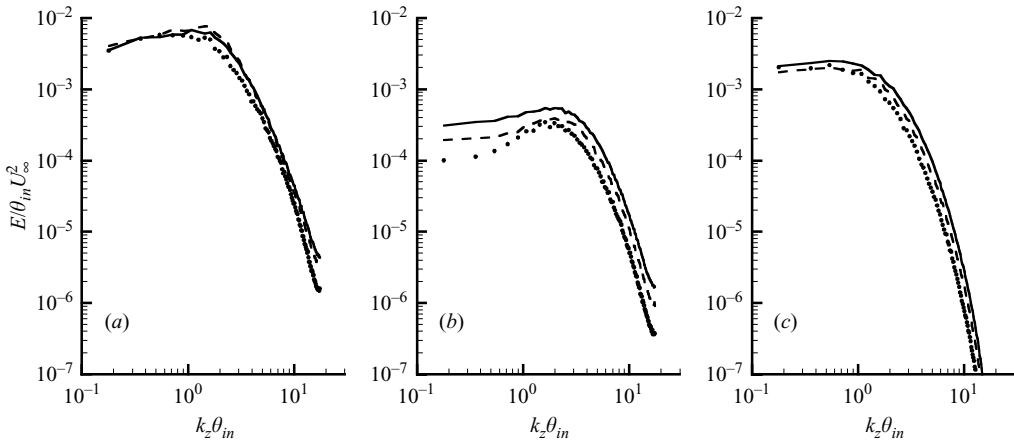
FIGURE 15. One-dimensional energy spectra at (\xi^+, y_o^+) = (300, 21) for Re_{\theta, in} = 670 : —, f^+ = 0.035 ; ---, SB ( f^+ = 0 ); ●, NB ( A^+ = 0 ). (a) E_{uu} ; (b) E_{vv} ; (c) E_{wv} .
