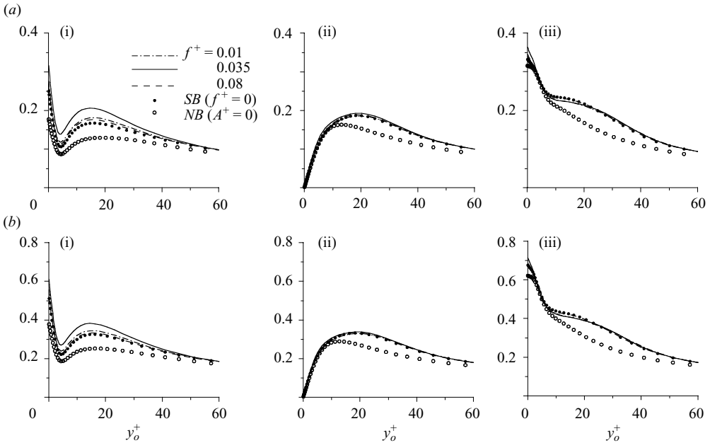
FIGURE 19. Root time-mean square of the vorticity fluctuations at \xi^+ = 300 . (a) Re_\theta = 300 ; (b) 670. (i) \omega'_{x,rms}\theta_{in}/U_\infty ; (ii) \omega'_{y,rms}\theta_{in}/U_\infty ; (iii) \omega'_{z,rms}\theta_{in}/U_\infty .
