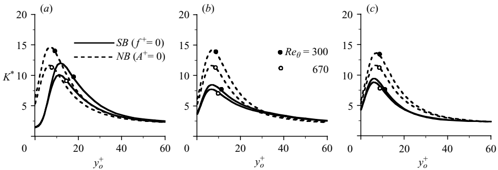
FIGURE 6. Energy partition parameter K^* = 2\overline{u'^2} / (\overline{v'^2} + \overline{w'^2}) . (a) \xi^+ = 0 ; (b) 500; (c) 1000.
