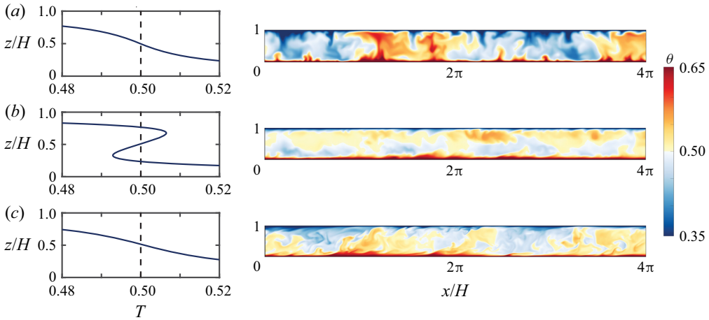
Figure 4. Mean wall-normal temperature profiles (left) and side view snapshots of temperature fields (right), i.e. streamwise cross-sections, for (a) Pr = 0.22 ; Re_w = 0 , (b) Pr = 0.22 ; Re_w = 4000 and (c) Pr = 1 ; Re = 4000 . For all right panels only x/H = 0-4\pi is shown for better visibility and y/H = 2\pi was chosen for the spanwise location at which periodic boundary conditions are employed.
