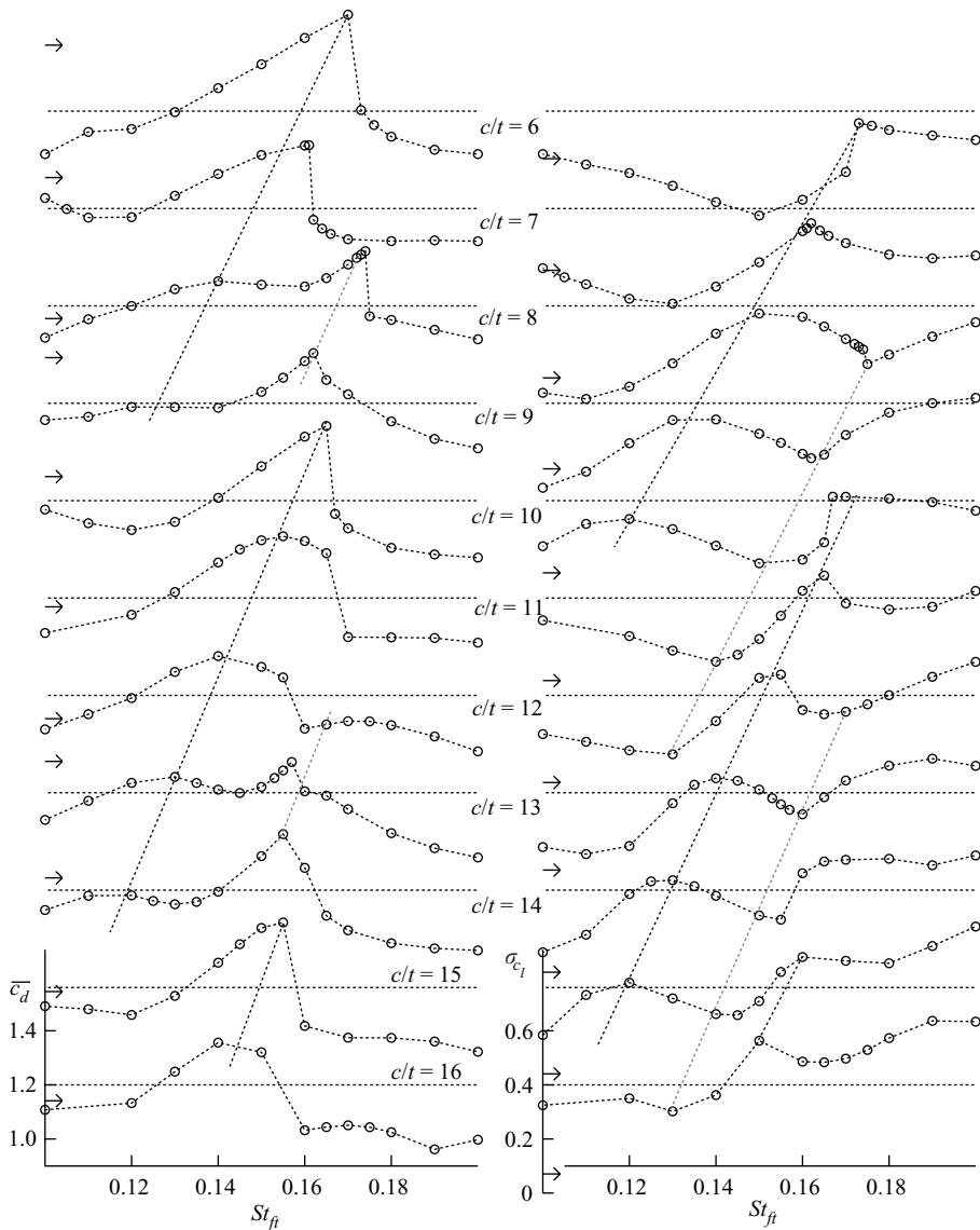
FIGURE 4. (a) Mean drag coefficient and (b) standard deviation of the lift coefficient as a function of forcing frequency for cylinders with 6 \leq c/t \leq 16 at Re = 400 and v_{pert} = 2.5\% . The arrows on the left show the mean drag coefficient and the standard deviation of the drag coefficient when no forcing is applied. The dashed black lines approximately connect the primary peaks and the dashed grey lines connect the secondary peaks.
