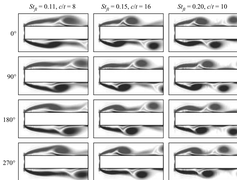
FIGURE 7. Vorticity plots of the leading-edge shedding at Re = 400 and v_{pert} = 2.5\% . Vorticity plots taken at 0^\circ , 90^\circ , 180^\circ and 270^\circ in the forcing cycle for cylinders with c/t = 8 , 16 and 10 at applied forcing frequencies of St_{ft} = 0.11 , 0.15 and 0.20 respectively.
