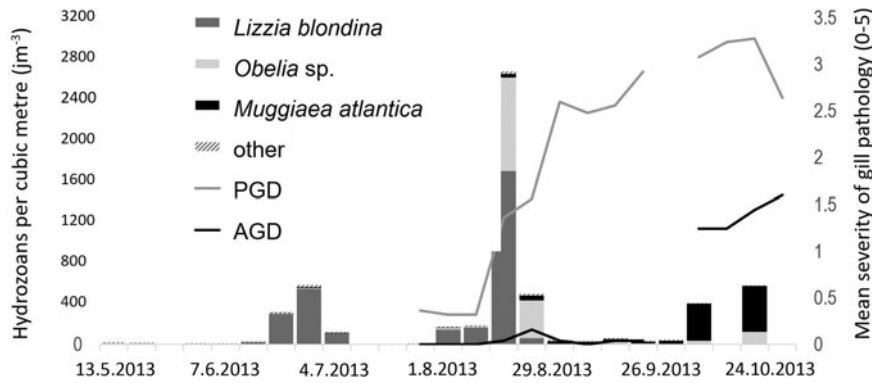
Fig. 12. Increase in PGD and AGD following bloom exposure. A major increase in PGD followed a high-magnitude spike in populations of Obelia sp. and Lizzia blondina ; AGD also increased with lag.
