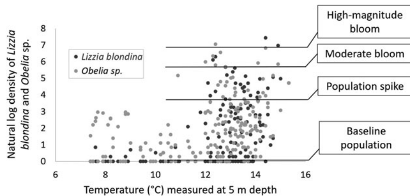
Fig. 10. Natural log of hydromedusan population density measured at sea surface temperature as measured at 5 m depth, with population magnitudes demarcated. Lizzia blondina and Obelia sp. medusae are most likely to occur in both spike and bloom-level population density measures in water greater than 12^\circ\text{C} .
