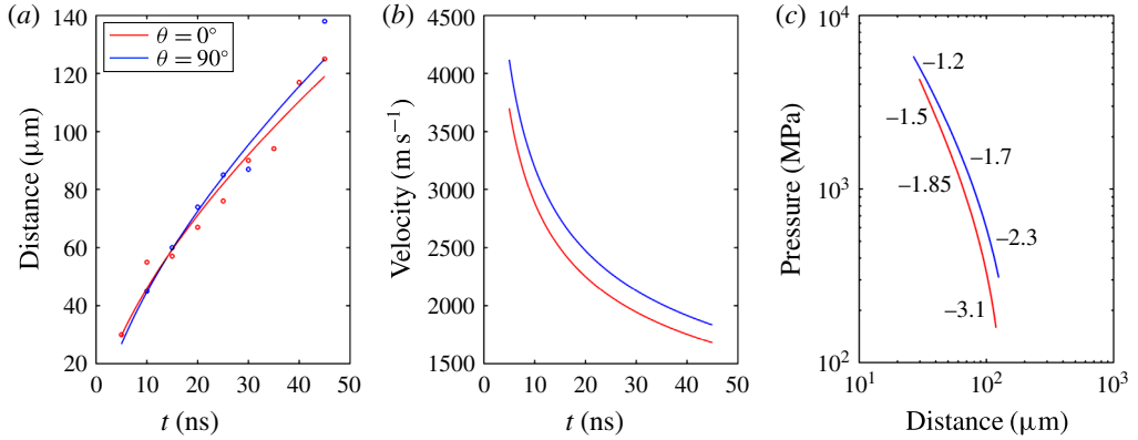
FIGURE 11. (Colour online) (a) The distance between plasma and shock front versus the elapsed time. (b) The velocity of the shock wave versus the elapsed time. (c) The pressure of the shock wave versus the distance between the plasma and shock front. The inserted numbers indicate the local slope of the corresponding curve.
