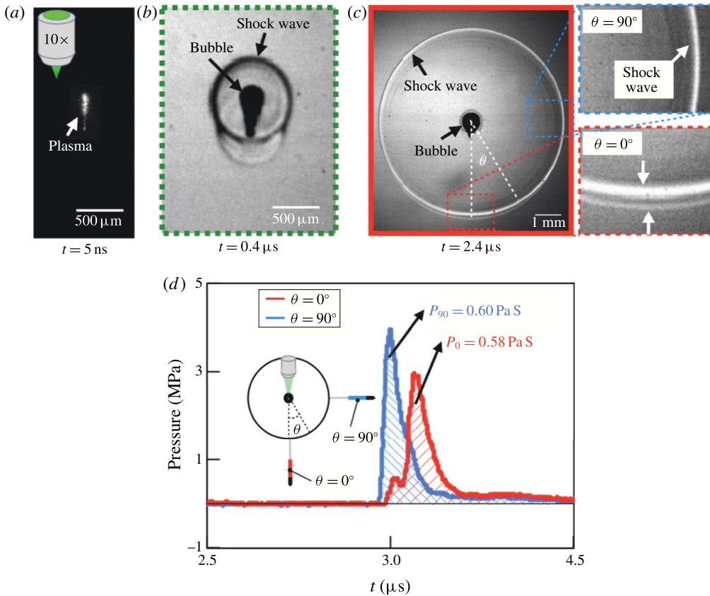
FIGURE 3. (Colour online) Measurement results for a laser-induced underwater shock wave obtained with a 10\times objective lens. (a) Plasma luminescence at t = 5 ns after the laser is fired. The image is captured by an ultra-high-speed video camera at 200 Mfps. (b) Shock waves and bubbles at t = 0.4 \mu\text{s} imaged with an ultra-high-speed video camera at 5 Mfps. (c) Shock waves at t = 2.4 \mu\text{s} measured with an ultra-high-speed video camera at 5 Mfps. Enlarged images for the areas of \theta = 0^\circ and \theta = 90^\circ are also presented. (d) Shock pressure measured by the two hydrophones arranged at \theta = 0^\circ (red line) and \theta = 90^\circ (blue line) with respect to the laser direction. Integrations for the pressure with respect to the elapsed time indicate pressure impulses.
