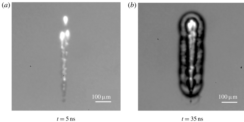
FIGURE 1. Snapshots of (a) a collection of plasmas in a conical region with 10\times objective, 6.9 mJ and (b) a collection of shock waves originated from plasmas. Time t denotes the elapsed time from the start of illumination with the laser pulse.
