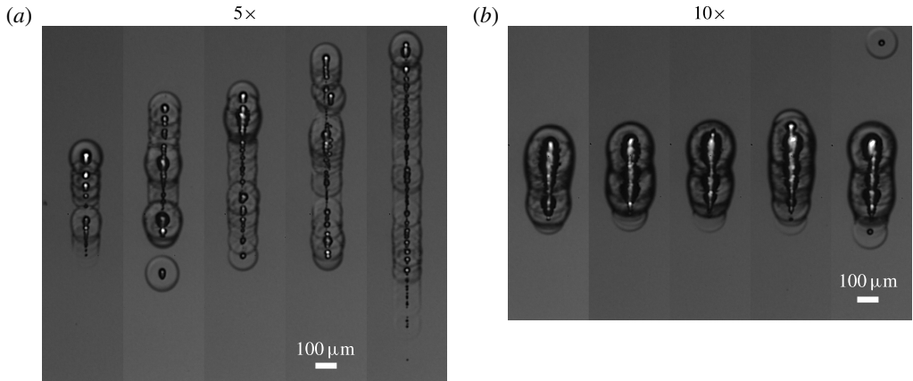
FIGURE 8. Snapshots of laser-induced bubbles and shock waves with 5 \times , 10 \times , 6.9 mJ, t = 50 ns. These results are obtained under the same conditions.
