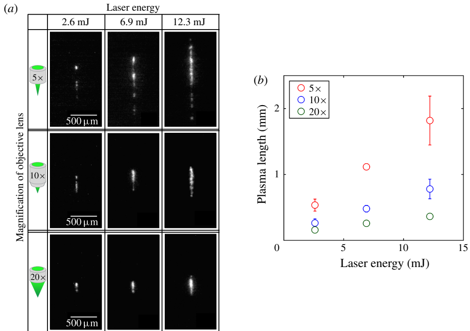
FIGURE 7. (Colour online) (a) Plasma formation under all experimental conditions (Magnification of objective lens: 5 \times , 10 \times , 20 \times . Laser energy: 2.6, 6.9 and 12.3 mJ). The plasma shape is the most elongated with an input energy of 12.3 mJ and the 5 \times objective lens, whereas it is rather spherical with an input energy of 2.6 mJ and the 20 \times objective lens. (b) Length of plasma as a function of the laser energy. The circle plot and error bar show respectively the mean and the standard deviation in 5 trials. Red, blue and green colour bar represent the microscope objective of 5 \times , 10 \times and 20 \times , respectively.
