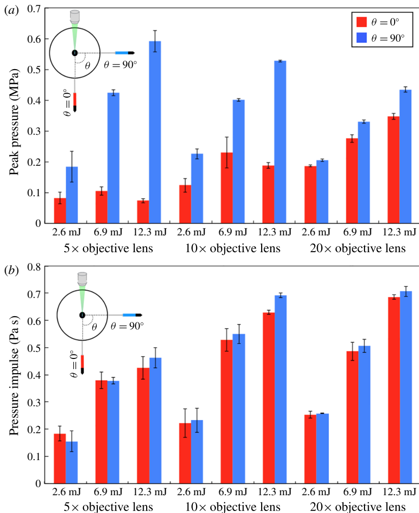
FIGURE 5. (Colour online) (a) Peak pressure of a laser-induced underwater shock wave measured at \theta = 0^\circ and \theta = 90^\circ for all the experimental conditions. Each presented value is a mean of three measurements and the error bars show the standard deviations. (b) Pressure impulse of a laser-induced shock wave measured at \theta = 0^\circ and \theta = 90^\circ for all the experimental conditions.
