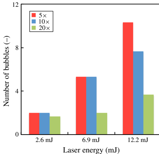
FIGURE 9. (Colour online) Number of bubbles of as a function of the laser energy. Each colour bar represents the result of one pulsed laser. Red, blue and green colour bars represent the microscope objective of 5 \times , 10 \times and 20 \times , respectively.
