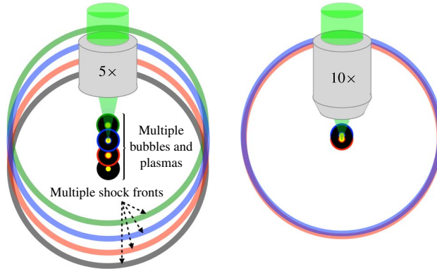
FIGURE 6. (Colour online) Schematic of a multiple structure model for a laser-induced underwater shock wave. Multiple plasmas emit multiple bubbles and spherical shock waves. The shock pressure at a certain point is the sum of the spherical shock pressures that reach the same point.
