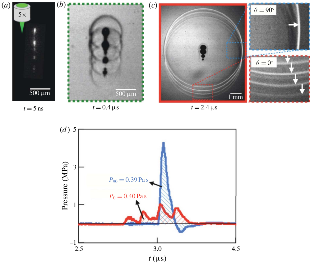
FIGURE 4. (Colour online) Measurement results for a laser-induced underwater shock wave obtained with a 5\times objective lens. Captions for (a–d) are the same as those in figure 3.
