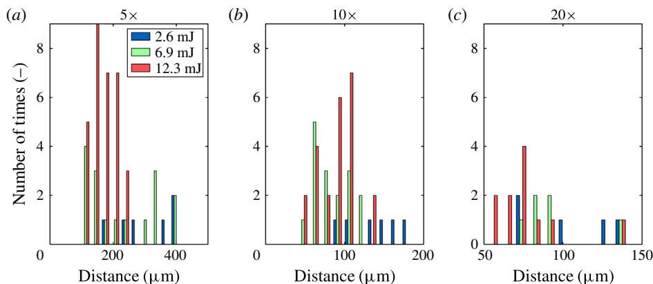
FIGURE 10. (Colour online) Histogram of the distances between bubble centres. Vertical axis is number of times that a certain distance emerges for all experiments; (a–c) show the histogram of the microscope objective of 5×, 10× and 20×, respectively. The colour of the bar represents the energy of a pulsed laser. The blue, green and red bars relate to 2.6, 6.9 and 12.3 mJ, respectively.
