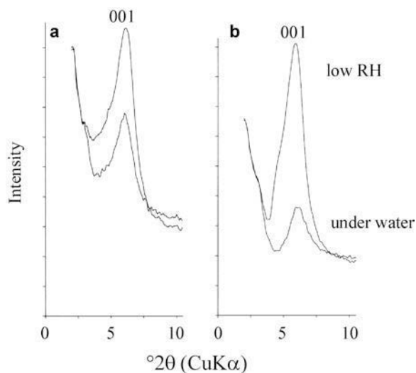
Figure 3. XRD patterns of \sim 100 nm thick PDPA/Laponite RD (a) and PDPA/montmorillonite (b) multilayer films under different environmental conditions: upper scans were taken at 23% RH (Laponite) and 25% RH (montmorillonite), and the lower scans were taken with the films under a film of water. The vertical axes in (a) and (b) both show the square root of intensity, but are plotted on different scales.
