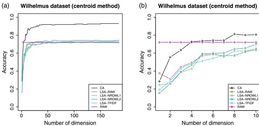
Figure 10. Accuracy versus the number of dimensions (centroid method) for CA, RAW, LSA-RAW, LSA-NROWL1, LSA-NROWL2, and LSA-TFIDF with Wilhelmus dataset.
