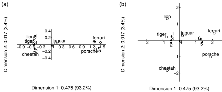
Figure 2. The data of Table 1 using CA for (a) symmetric map and (b) asymmetric map.
