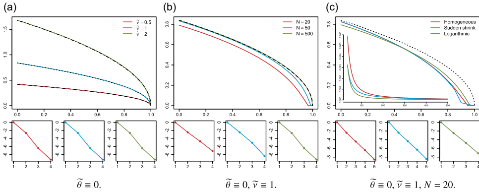
FIGURE 1. The picture shows a comparison between the exact OSB of a BB and its numerical computation, which is obtained by setting \tilde{\theta} \equiv 0 and taking a constant volatility \tilde{\nu} in the OU representation (65). For the images on top, the solid colored lines represent the computed OSBs for the different choices of the volatility coefficient \tilde{\nu} (image (a)), the partition length N (image (b)), and the type of partition considered (image (c)). The black dashed, dotted, and dashed-dotted lines represent the OSB of a BB associated with the different values of \tilde{\nu} . Specifications are shown in the legend and caption of each image. Image (c) accounts for a subplot that shows, as a function of the partition size N ( x -axis), the evolution of the relative L_2 error between the various computed boundaries and the true one ( y -axis). The smaller images at the bottom show the log-errors \log_{10}(d_k) between consecutive boundaries for each iteration k = 1, 2, \dots of the Picard algorithm.
