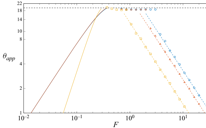
Figure 2. Plots of apparent wake angle against the Froude number. The solid curve represents Method I defined in § 2.5 using a 20 % cutoff height. The low-Froude-number results only consider the transverse waves of the stationary phase approximation. The apparent wake angles calculated from Method II are given by the marks with the large-Froude-number approximation given by the dashed line. The blue, red and yellow colours denote flow past a submerged source, submerged doublet and applied pressure distribution, respectively.
