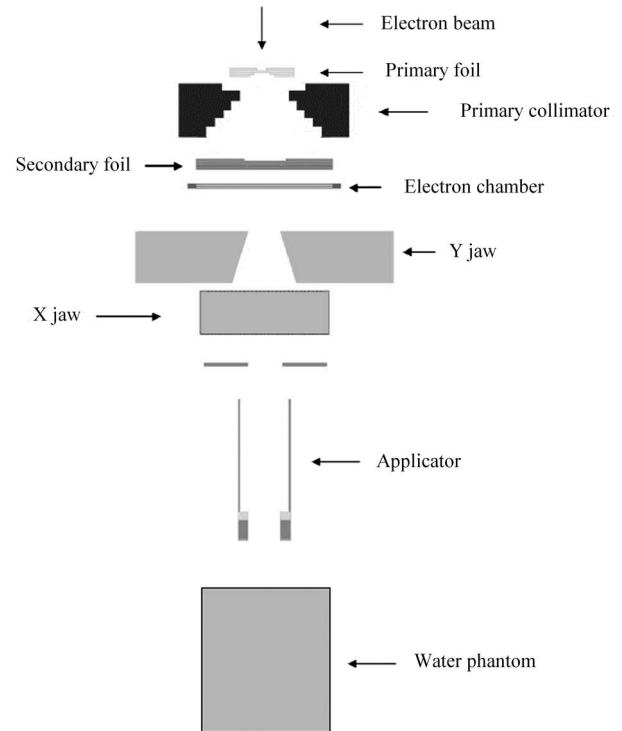
Figure 1. Geometry of head of Siemens Primus linac in electron mode as well as the water phantom.
