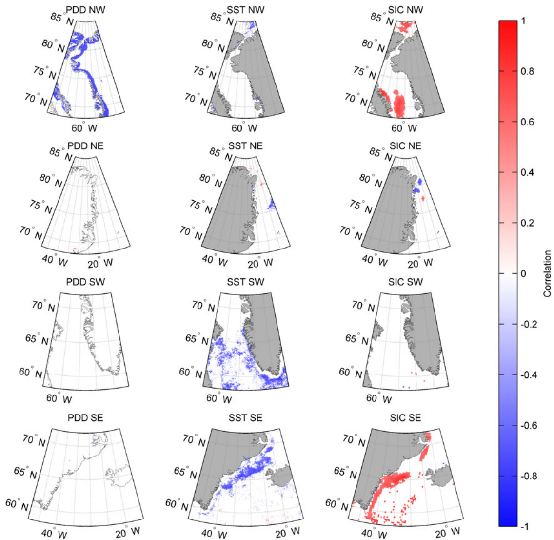
Fig. 6. Maps of correlations with confidence above 95% for the comparison between the normalized average area change of the glaciers from each region and the three climate parameters.
