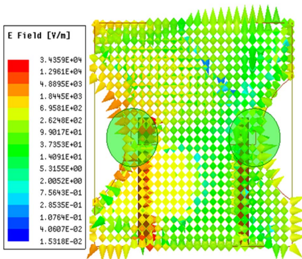
Figure 6. Simulated E-field distribution of ground plane at A_R = 8 mm.
