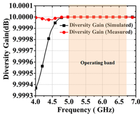
Figure 22. Comparison between simulated and measured DG.
