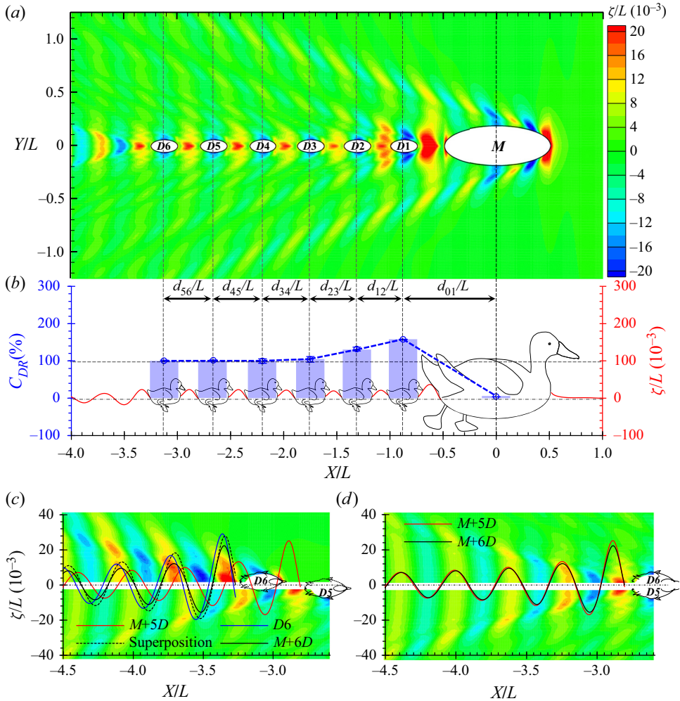
Figure 4. Optimum swimming formation by a mother duck ( M ) followed by duckling(s) in a clutch of n ( nD ). (a) Wave pattern by M + 6D in an optimum formation. Here D_n represents the n th duckling in the formation. (b) Wave drag reduction of each individual (blue dash line and columns). The red solid curve is the wave profile on the centre line behind the mother duck. Here d_{n,n+1} is the separation between two adjacent individuals, where the subscript n = 0 represents the mother duck. The virtual ducklings are put in the positions of minimum wave drag. The error bar in panel (b) gives an indication of the errors induced by numerical discretization. Panels (c) and (d) show a decomposition of the wave patterns and wave profiles. (c) The background contour represents the wave pattern. Upper half: waves generated by a single duckling swimming independently at D_6 . Lower half: waves generated by M + 5D . The curves are the wave profiles at the centre line behind ducklings. Red solid curve: wave profile behind the 5th duckling in an optimum M + 5D formation. Blue solid curve: wave profile behind a single duckling swimming independently at D_6 . Black dash curve: superposition of the red and blue solid curves. Solid black curve: wave profile behind the 6th duckling in an optimum M + 6D formation. (d) Lower half of the contour and the red solid curve are the same as those defined in panel (a). Upper half of the contour is the wave pattern of M + 6D shifted upstream by d_{56}/L . Shifting the black solid curve in panel (c) upstream by d_{56}/L , we can obtain the black curve in panel (d).
