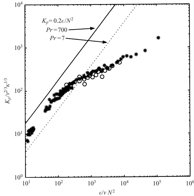
FIGURE 8. Normalized experimental diffusivity results, K_\rho/v^{2/3}k^{1/3} and the normalized prediction for K_\rho due to Osborn (1980) vs. turbulence intensity \epsilon/vN^2 ; *, water experiments; O, water–glycerol experiments; —, Osborn (1980), for Pr = 700 ; ···, Osborn (1980), for Pr = 7 .
