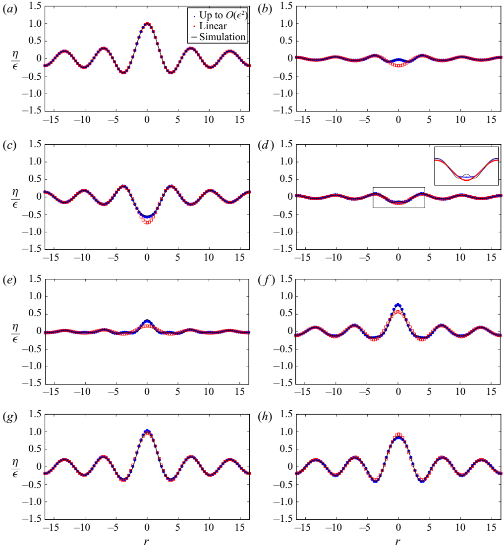
FIGURE 7. (a–h) Comparison of the (non-dimensional) interface shape \eta/\epsilon versus radius r at various (non-dimensional) time instants for \epsilon = 0.5 : (a) t = 0 ; (b) t = 1.228 ; (c) t = 1.658 ; (d) t = 3.133 ; (e) t = 3.378 ; (f) t = 3.685 ; (g) t = 4.177 ; (h) t = 4.607 . Simulation profiles (—, black), linear theory ( \square , red) and weakly nonlinear theory ( \bullet , blue). Dimple formation initiates in panel (b), is suppressed as the trough reaches its lowest point and reappears with significant shortening in scale as seen in inset of panel (d). Weakly nonlinear model qualitatively and significantly improves over the linearised model in this regime. For parameters, see case 1 in table 3, grid (a).
