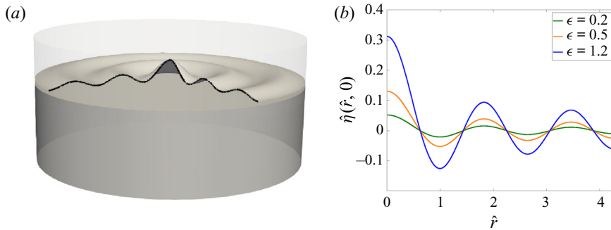
FIGURE 1. (a) Initial condition: the black line depicts cross-section of the perturbed interface at \hat{t} = 0 . The interface initially is \hat{\eta}(\hat{r}, 0) = a_0 J_0(k\hat{r}) where J_0 is the zeroth-order Bessel function of the first kind, k is the wavenumber, a_0 is the perturbation amplitude and \hat{r} is the radial coordinate. The liquid (in grey) is quiescent initially. (b) The effect of changing the wave steepness parameter \epsilon \equiv a_0 k on the initial perturbation. Here \epsilon is a non-dimensional measure of the maximum slope of the initial perturbation. A wave with \epsilon \ll 1 has an amplitude much smaller than its wavelength and can be described by linear theory. Jets form at the axis of symmetry for moderate to high values of \epsilon ( > 0.5 typically) and are nonlinear phenomena. We use \epsilon as a small parameter in our perturbative expansion.
