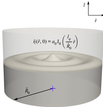
FIGURE 3. Three-dimensional visualisation of surface perturbation (grey). Surface perturbation imposed at \hat{t} = 0 leads to a jet at the end of one oscillation for sufficiently large \epsilon . The coordinate system is centred at the axis of symmetry and \hat{z} is measured from the unperturbed free surface.
