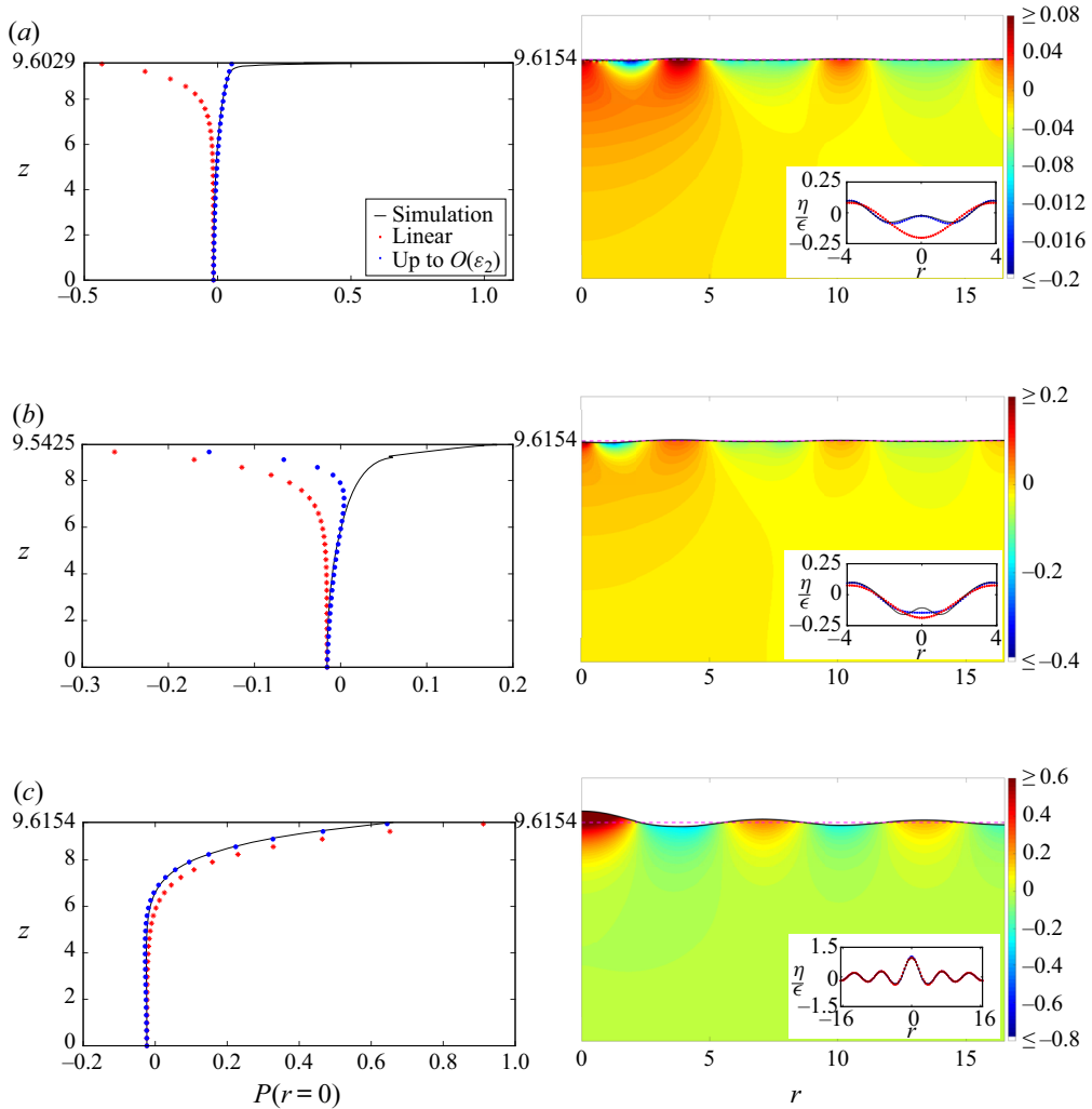
FIGURE 10. Left panels: (non-dimensional) pressure profiles P(r, z, t) at the axis of symmetry r = 0 at various time instants for \epsilon = 0.5 . Right panels: pressure contours from numerical simulations. The dashed line on the contour plots represents the depth of the unperturbed liquid at t = 0 . The insets depict the instantaneous interface shape. As the weakly nonlinear theory has been derived using a Taylor series expansion about the unperturbed state for the liquid side only, we plot data at most up to the (scaled) unperturbed depth ( z = 9.6154 ). For parameters, see case 1 in table 3, grid (a). (a) Time t = 1.228 ; pressure profiles (left) and contours (right) at the onset of dimple formation. (b) Time t = 3.133 ; pressure profiles and contours with a sharper and narrower dimple. (c) Time t = 4.177 ; pressure profiles and contours when the jet is close to its maximum height.
