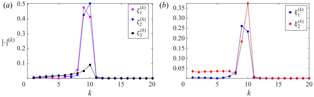
FIGURE 4. Here, \zeta_1^{(k)} , \zeta_2^{(k)} , \zeta_3^{(k)} and \xi_1^{(k)} , \xi_2^{(k)} for q = 5 as a function of k . After k = 12 , the values are quite small permitting truncation of the infinite series in (2.36) and (2.37).
