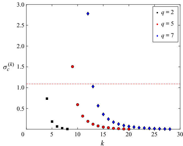
FIGURE 18. Critical values \sigma_c^{(k)} for various choices of the primary mode q . In this study we have chosen \sigma = 1.086 (dotted red line) which is far from the two neighbouring critical values of sigma, indicated by red dots for q = 5 .
