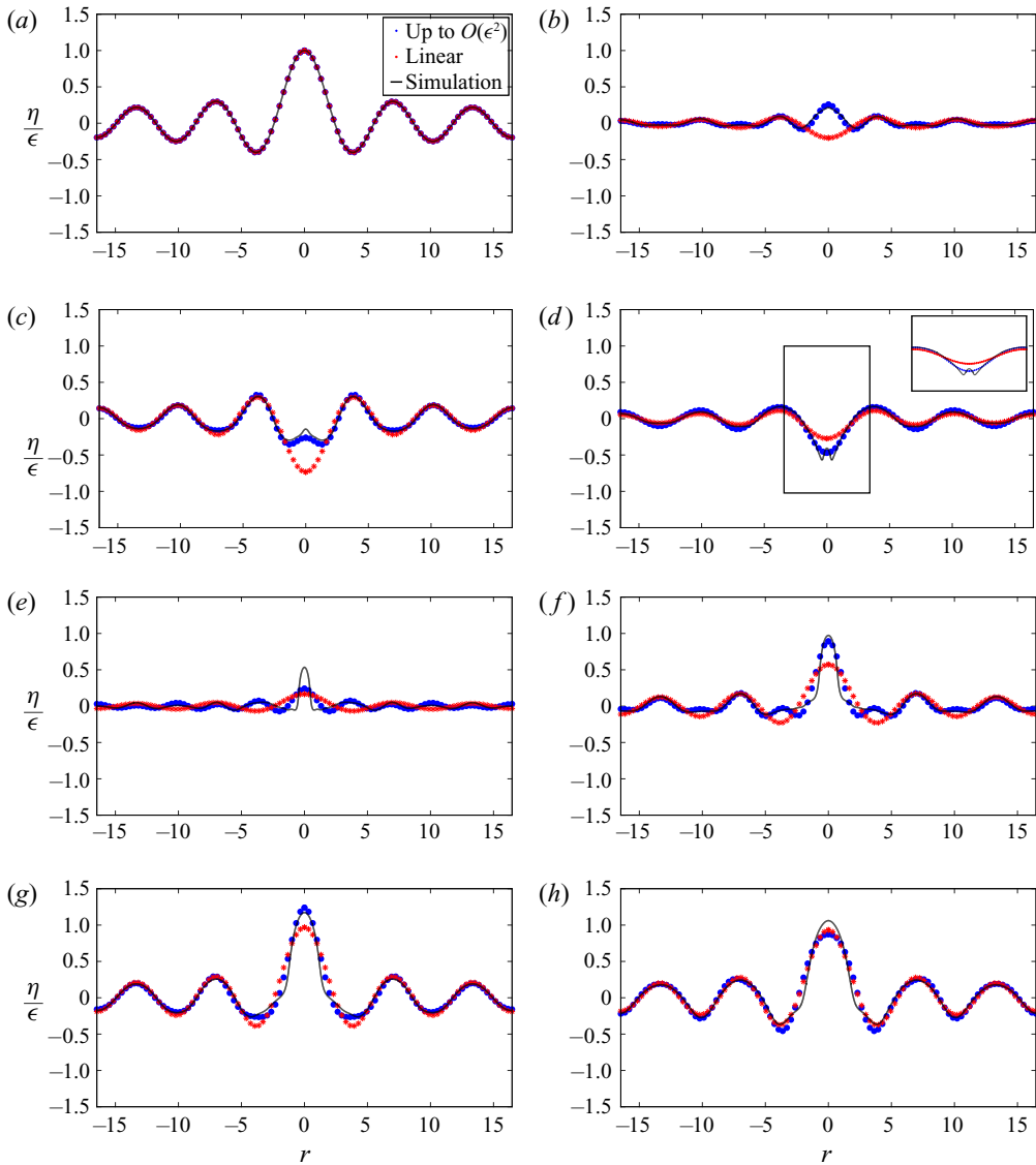
FIGURE 8. (a–h) Comparison of the (non-dimensional) interface shape \eta/\epsilon versus radius r at various (non-dimensional) time instants for \epsilon = 1.2 : (a) t = 0 ; (b) t = 1.228 s; (c) t = 1.658 ; (d) t = 3.071 ; (e) t = 3.378 ; (f) t = 3.685 ; (g) t = 4.177 ; (h) t = 4.607 . Simulation profiles (—, black) are compared with linear ( \square , red) and weakly nonlinear predictions ( \bullet , blue). Dimple initiation is well captured by the nonlinear theory in panel (c) but not later on in panel (d) where the dimple becomes sharper and more pronounced, see inset. The thinning of the neck of the jet is not captured by the nonlinear model in panel (e). Near maximum overshoot, the jet shape near r = 0 is well described by theory, see panel (f,g). For parameters see case 5 in table 3, grid (b).
