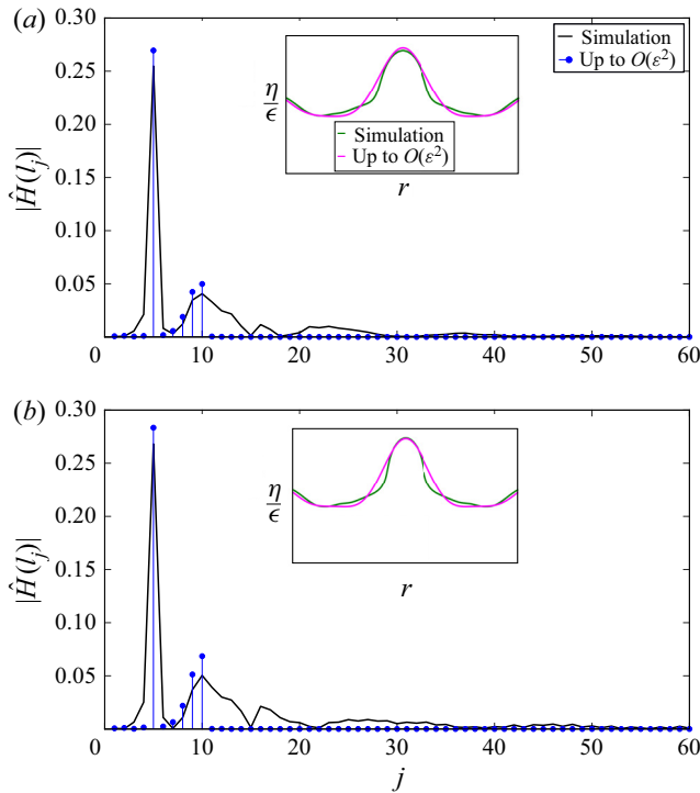
FIGURE 17. Here \hat{H}(j; \hat{t}_0) versus j when the jet is at its maximum height: (a) \epsilon = 1.2 ; (b) \epsilon = 1.3 . As seen from the jet shape in the insets, the nonlinear model estimates the maximum height of the jet well but not the ‘shoulder’ of the jet, instead developing a broader base. It is concluded that in order to predict maximum height, one needs to estimate potential energy in modes up to j = 10 only which the theory does well. However, for resolving the jet ‘shoulder’, one has to estimate the potential energy in modes > j = 10 accurately which the O(\epsilon^2) theory cannot capture. Here \hat{t}_0 = 0.067 s.
