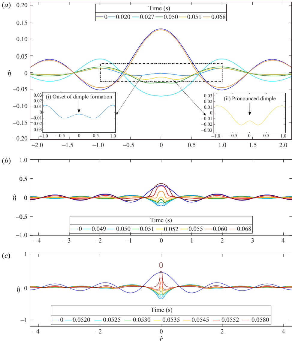
FIGURE 2. Results from numerical simulations: temporal evolution of the interface for (a) \epsilon = 0.5 , (b) \epsilon = 1.2 and (c) \epsilon = 1.7 . (a) A dimple appearing at the base of the wave trough is a nonlinear event and signals impending jetting. This is seen more clearly in panels (b,c) where \epsilon is chosen to be larger and produces a jet which overshoots the initial perturbation at \hat{r} = 0 and also ejects a drop in panel (c); note the slender jet. (a) Dimple formation with time for \epsilon = 0.5 . (b) Pronounced dimple, jet formation and overshoot at \hat{r} = 0 for \epsilon = 1.2 . (c) Pronounced dimple, slender jet, overshoot, drop ejection for \epsilon = 1.7 .
