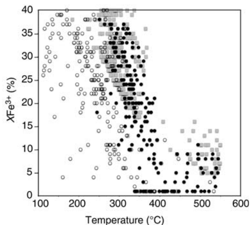
FIG. 6. Estimated TFe^{3+} Vidal and \chi Fe^{3+} pairs for low- and medium-pressure samples (open circles), high-pressure samples (black circles) and the samples from Grosch et al. (2012) (grey squares).
