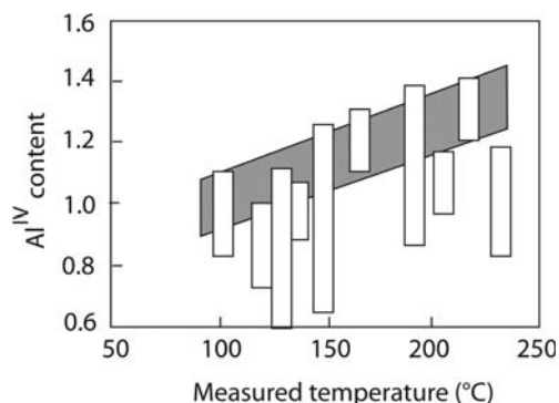
FIG. 12. Range of crystal-rim \text{Al}^{\text{IV}} content (white boxes) of Gulf Coast chlorites vs. measured temperatures. The grey area underlines the range of maximum \text{Al}^{\text{IV}} content, which is assumed to represent the closest approach to equilibrium composition (after Bourdelle et al. , 2013b).
