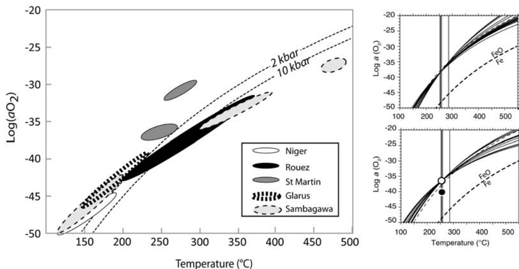
FIG. 8. Left: Ranges of \text{Log}(a_{\text{O}_2}) conditions calculated for the samples used to compute Fig. 7 at the temperature and X_{\text{Fe}^{3+}} contents estimated from the Chl-Qtz- \text{H}_2\text{O} equilibrium conditions. Dashed lines: hematite-magnetite- \text{O}_2 equilibrium calculated using the thermodynamic properties of Berman (1988) and unit activities of Ht and Mt. Right: Sample calculation at 2 kbar for a Rouez sample using reactions 8–20 (upper) or 26–40 (lower). The vertical lines correspond to oxygen- and magnetite-free reactions 1, 5, 6 and 7 used to compute Figs 5–7, which converge at \pm 30^\circ\text{C} . The circles in the lower figure represent values calculated with (\Delta H^{\circ}f) ferri-Sud constrained with the chlorite-magnetite-quartz-water equilibria 8–20 (open circle) or estimated as \Delta H^{\circ}f(\text{Mg-sudoite}) - \Delta H^{\circ}f(\text{corundum})/2 + \Delta H^{\circ}f(\text{hematite})/2 (filled circle) (see Table 1 and text).
