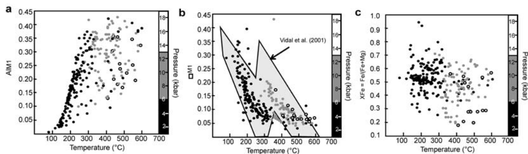
FIG. 3. Al on M1 (a), vacancy on M1 (b) and X_{Fe} of chlorite (c) as a function of temperature and pressure (after Lanari et al. , 2014) assuming that Fe_{Total} = Fe^{2+} . AlM1 and \square M1 are proportional to the amount of amesite and sudoite end-members respectively (AlM1 = 1 for pure amesite, \square M1 = 1 for pure sudoite, AlM1 = \square M1 = 0 for amesite-free and sudoite-free chlorite). The grey area in part b encompasses the vacancy contents reported by Vidal et al. (2001).
