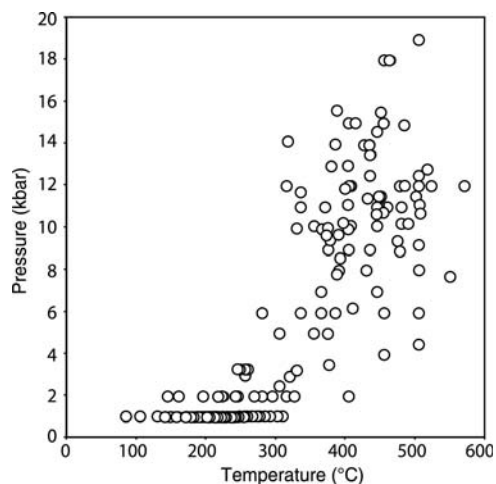
FIG. 1. Pressure and temperature conditions of the samples used in the present study
