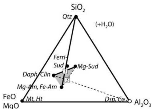
FIG. 2. Composition of the end-members and range of chlorite composition (grey area) considered in the present study plotted in a SiO_2 - FeO - MgO - Al_2O_3 ternary diagram. The intersection of the continuous and dashed lines corresponds to reactions 1 and 3 listed in the text.
