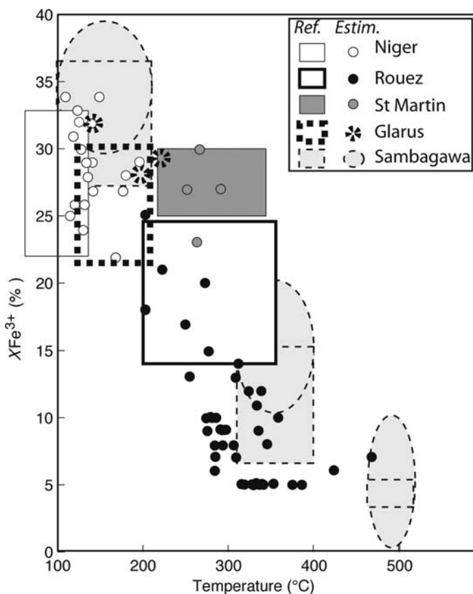
FIG. 7. Boxes: measured \chi Fe^{3+} and reference temperatures. Symbols: T_{\text{maximum}}-\chi Fe^{3+} minimum pairs calculated to obtain convergence ( \pm 30^\circ C ) of equilibria 1, 8, 9 and 10 with the thermodynamic model of Vidal et al. (2006).
