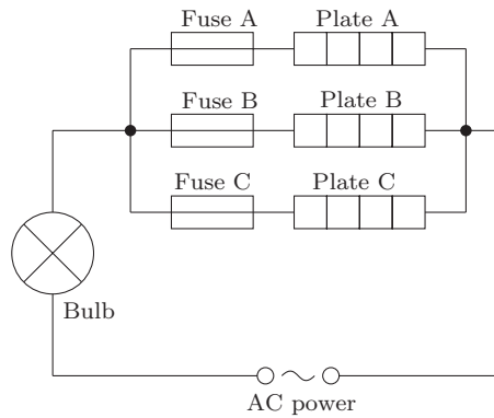
Fig. 2. Schematics of the electronic circuit we want to diagnose.
