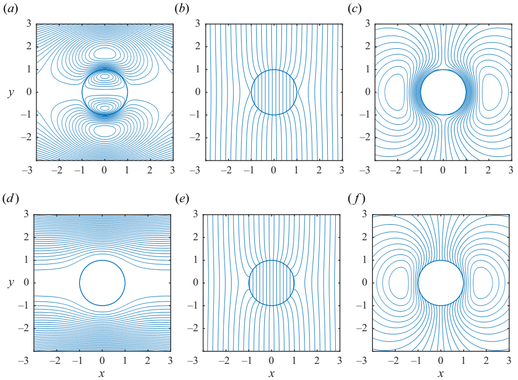
Figure 10. Streamlines ( a,d ), electrostatic potential perturbation ( b,e ) and co-cation-concentration perturbation ( c,f ) for stationary drops subjected to an electric field (from left to right): \zeta^* = 0.5 , \kappa a = 1 , \eta_i/\eta_o = 0.01 ( a-c ), 100 ( d-f ). Other parameters are the same as in figure 4.
