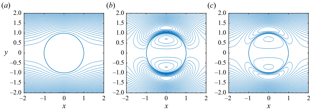
Figure 11. Streamlines (in the drop frame) for a low-viscosity drop subject to ( a ) uniform (left-to-right) far-field flow; ( b ) uniform (left-to-right) electric field; and ( c ) force-free electrophoresis: \zeta^* = 1 , \kappa a = 5 , \eta_i/\eta_o = 0.01 . Other parameters are the same as in figure 4.
