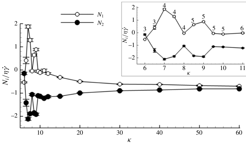
FIGURE 22. Effect of confinement \kappa on normal stress differences N_1/\eta\dot{\gamma} (○) and N_2/\eta\dot{\gamma} (●) at \phi_{bulk} = 0.4 and \mu_d = 0 in the range 6 \leq \kappa \leq 60 . (Inset: range 6 \leq \kappa \leq 11 ; the numbers labelling the circles indicate the number of layers).
