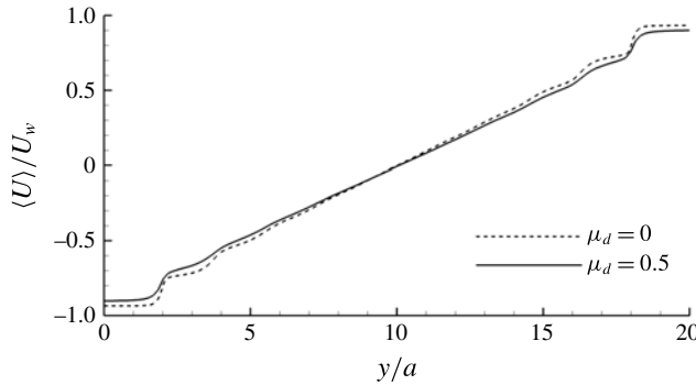
FIGURE 8. Particle-phase axial velocity \langle U(y)\rangle/U_w for frictionless particles \mu_d = 0 (dotted lines) and frictional particles \mu_d = 0.5 (solid lines). Simulations at \phi_{bulk} = 0.4 and \kappa = 20 .
