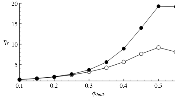
FIGURE 12. Relative viscosity \eta_r as a function of volume fraction ( \kappa = 20 ) for friction coefficients \mu_d = 0 (○) and \mu_d = 0.5 (●).
