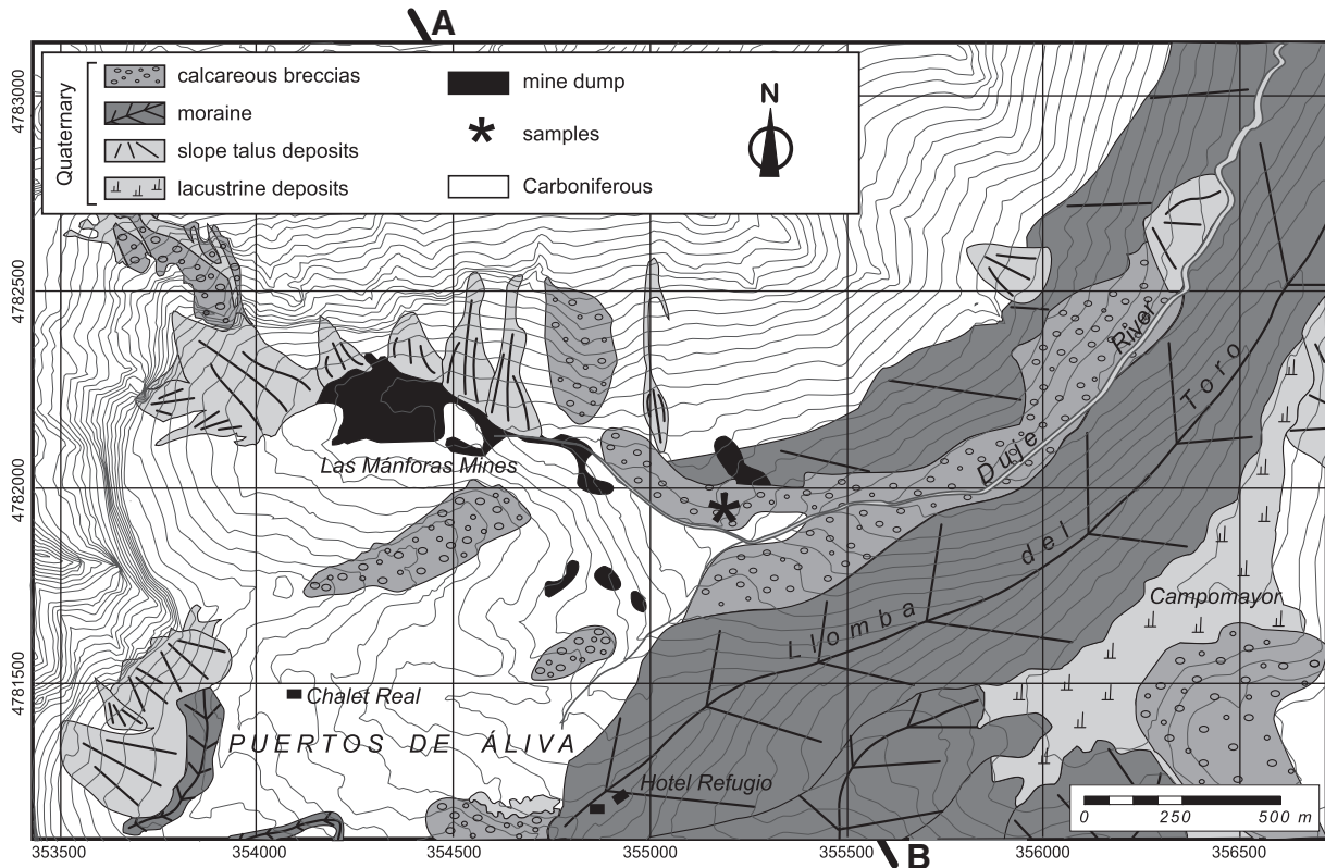
Figure 2. Geomorphological sketch showing the distribution of the Quaternary breccias in the Duje Valley and location of some relevant localities (A–B, cross-section in Fig. 3).
