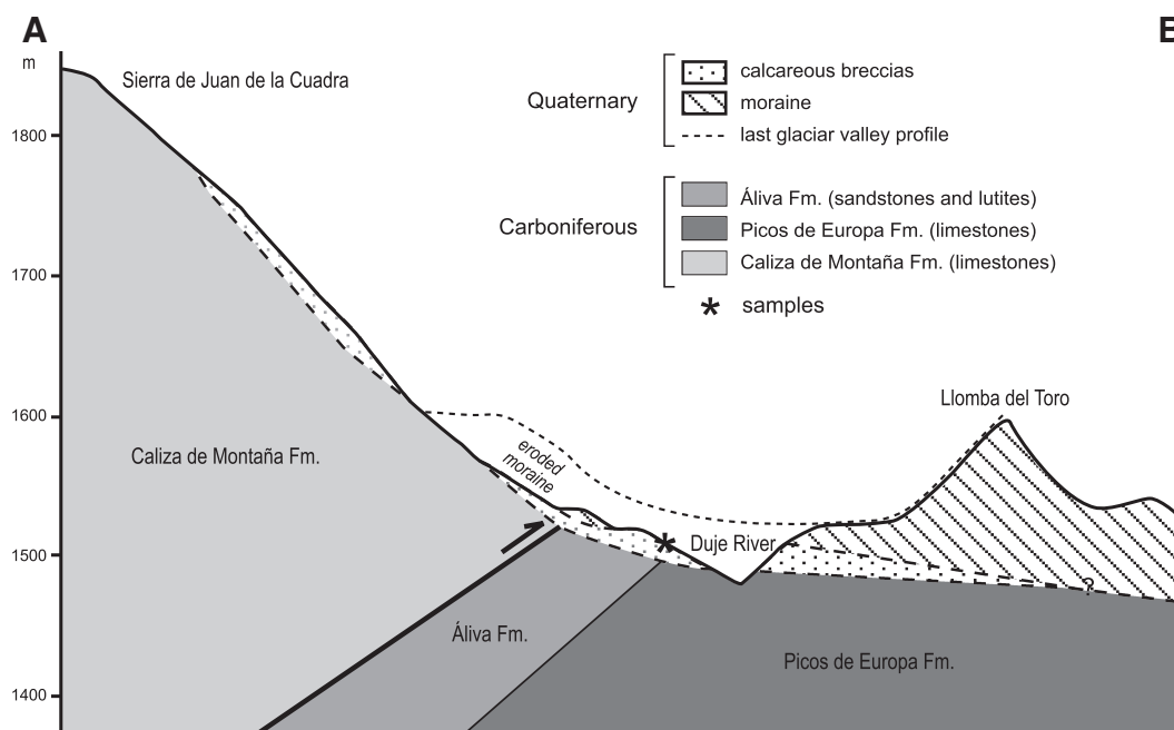
Figure 3. Cross-section of the Quaternary deposits observed in the upper part of the Dujé Valley.
