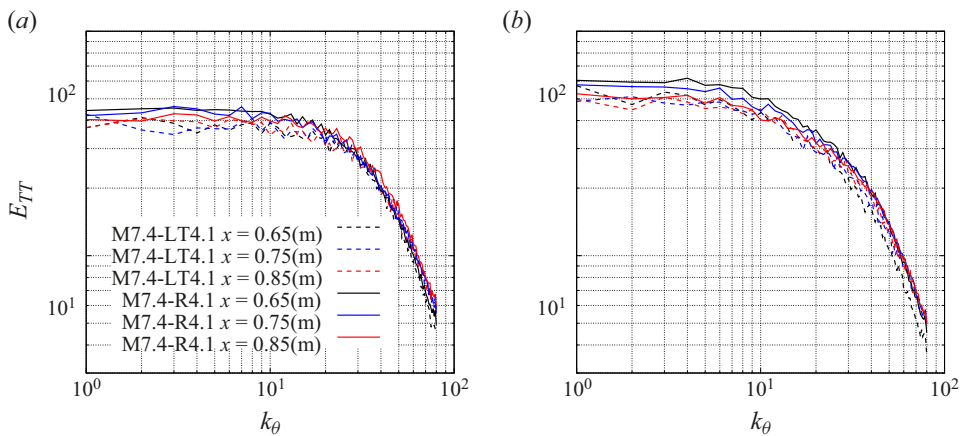
Figure 10. Comparison of one-dimensional spectra of temperature fluctuations in the azimuthal direction between the laminar-to-turbulent transition simulation M7.4-LT4.1 and the volumetric rescaling simulation M7.4-R4.1 for several x locations. The data are extracted at (a) y^* = 15 and (b) y^* = 300 .
