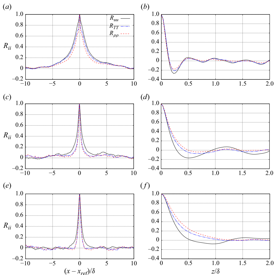
Figure 27. Two-point correlations of streamwise velocity, temperature and density components at x_{ref} = 0.8 m in the (a,c,e) streamwise and (b,d,f) azimuthal directions. The data are computed for (a,b) y^* = 5 , (c,d) y^* = 161 and (e,f) y^* = 784 . These y^* locations correspond to (a,b) y = 0.064 mm, (c,d) y = 1.9 mm and (e,f) y = 5.6 mm, respectively.
