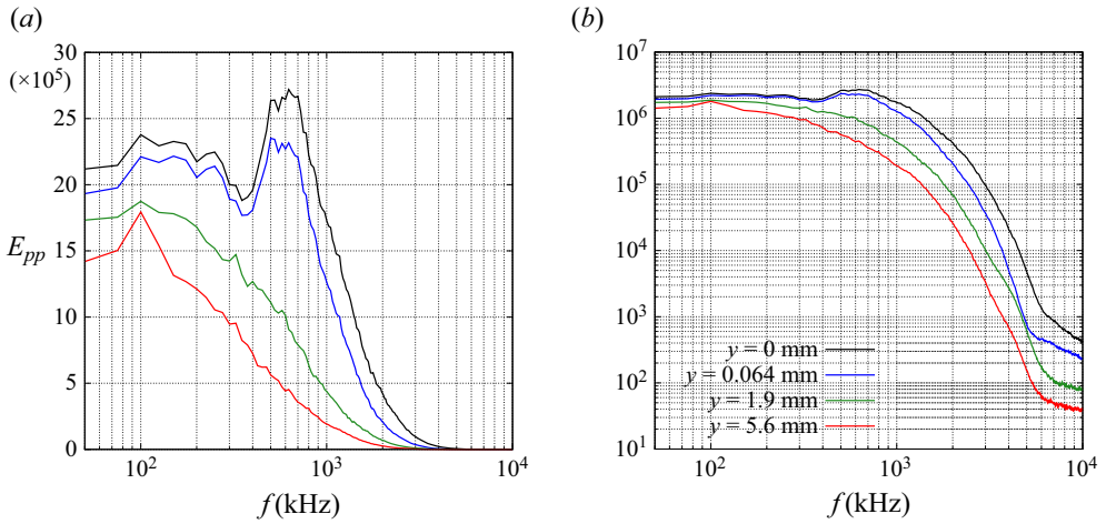
Figure 32. Energy spectra of pressure fluctuations in time at x = 0.85 m for the M7.4-R4.1 case for several y^* locations. The spectra are shown in (a) the linear scale and (b) the logarithmic scale.
