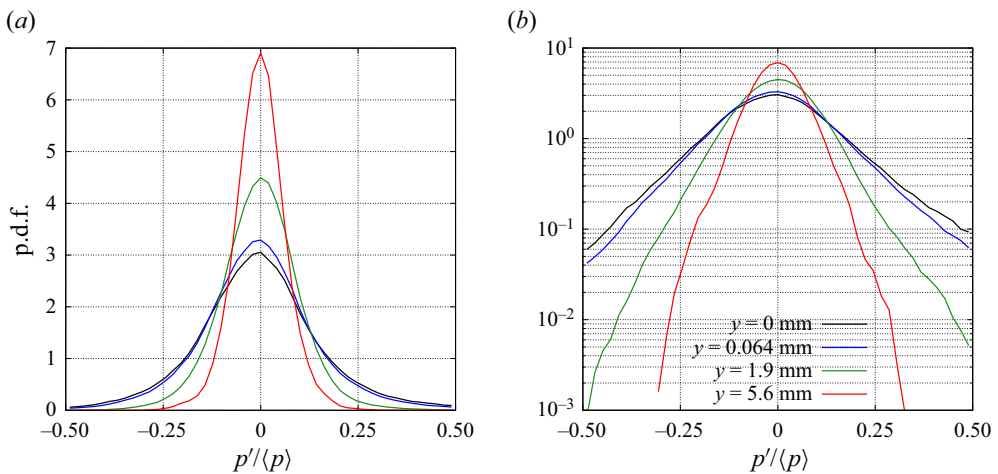
Figure 33. The p.d.f. of pressure fluctuations at x = 0.85 m for the M7.4-R4.1 case for several y^* locations. The data are shown in (a) the linear scale and (b) the logarithmic scale.
