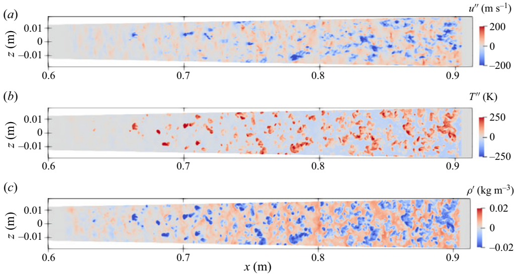
Figure 26. Instantaneous snapshot in the y = 5.6 mm ( y/\delta = 0.9 , y^* = 760 at x = 0.85 m) wall-parallel plane for M7.4-R4.1. Statistical fluctuation of (a) streamwise velocity, (b) temperature and (c) density.
