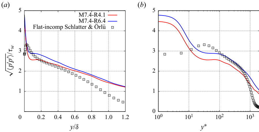
Figure 18. Pressure fluctuation correlations at x = 0.85 m as a function of (a) the outer scaling y/\delta and (b) the semi-local wall unit y^* . The DNS results of flat plate incompressible boundary layers by Schlatter & Örlü (2010) are also included.
