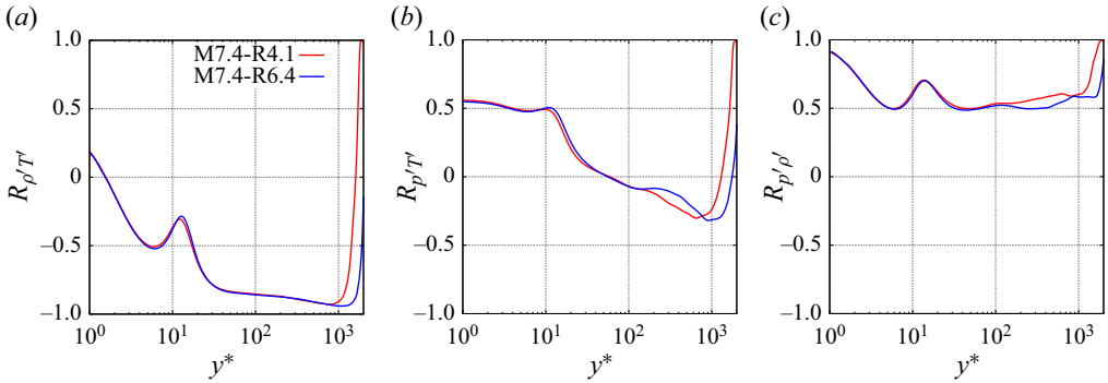
Figure 20. Correlation coefficients of (a) density–temperature, (b) pressure–temperature and (c) pressure–density at x = 0.85 m.
