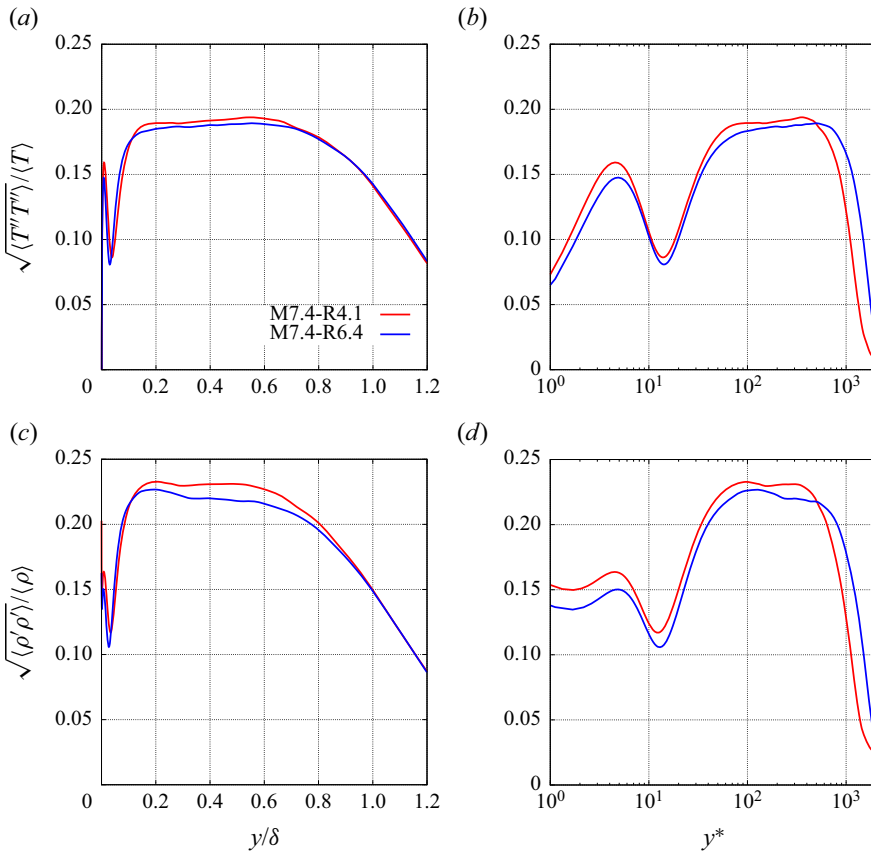
Figure 19. Fluctuation correlations of (a,b) temperature and (c,d) density at x = 0.85 m as a function of (a,c) the outer scaling y/\delta and (b,d) the semi-local wall unit y^* .
