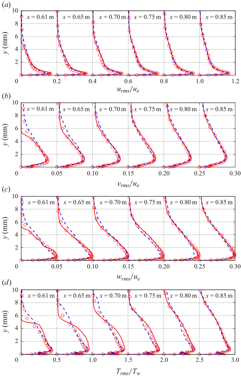
Figure 12. Fluctuation correlation profiles of (a) streamwise velocity, (b) wall-normal velocity, (c) spanwise velocity, (d) temperature for Re_m = 4.1 \times 10^6 \text{ m}^{-1} cases. Results of the volumetric rescaling simulation M7.4-R4.1 (red solid line) are compared with those of the laminar-to-turbulent transition simulation M7.4-LT4.1 (blue dashed line). Red circles are the result of backpropagating the variance profiles from x = 0.85 to x = 0.61 m, rescaling them vertically based on the boundary-layer height, serving as a reference for the local self-similar state of turbulence.
