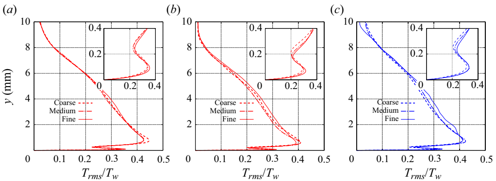
Figure 6. Grid sensitivity study for fluctuation correlations of temperature at x = 0.85 m in (a) M7.4-R4.1, (b) M7.4-R6.4 and (c) M7.4-LT4.1.
