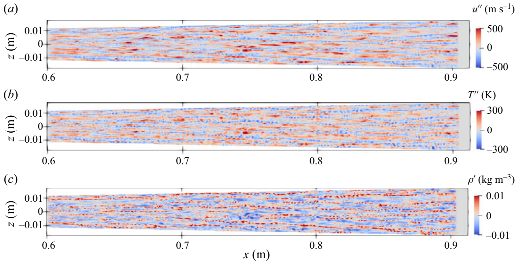
Figure 24. Instantaneous snapshot in the y = 0.064 mm ( y/\delta = 0.01 , y^* = 5 at x = 0.85 m) wall-parallel plane for M7.4-R4.1. Statistical fluctuation of (a) streamwise velocity, (b) temperature and (c) density.
