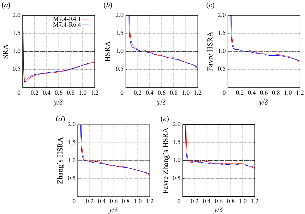
Figure 23. (a) The SRA relation of (5.4), (b) the HSRA of (5.6), (c) the Favre HSRA of (5.7), (d) Zhang's HSRA of (5.8) and (e) the Favre Zhang's HSRA of (5.10) at x = 0.85 m.
