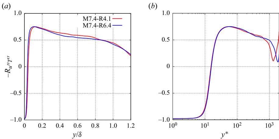
Figure 22. Temperature-velocity correlation coefficient at x = 0.85 m as a function of (a) the outer scaling y/\delta and (b) the semi-local wall unit y^* .
