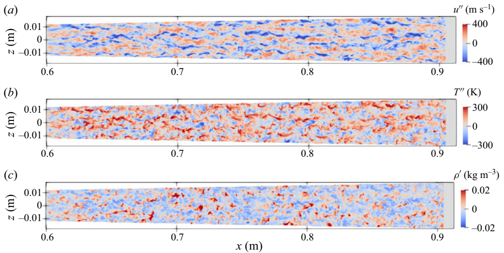
Figure 25. Instantaneous snapshot in the y = 1.9 mm ( y/\delta = 0.3 , y^* = 160 at x = 0.85 m) wall-parallel plane for M7.4-R4.1. Statistical fluctuation of (a) streamwise velocity, (b) temperature and (c) density.
