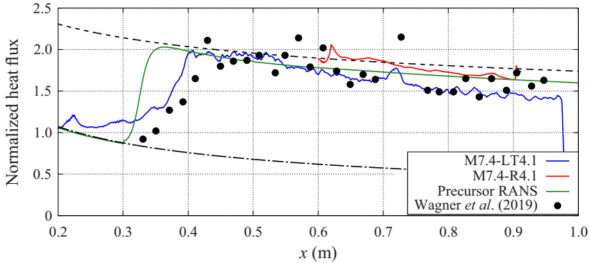
Figure 7. Comparison of wall-heat flux profiles between the volumetric rescaling simulation M7.4-R4.1 and the laminar-to-turbulent transition simulation M7.4-LT4.1. Data of the precursor RANS and the experiment by Wagner et al. (2019) are also included. Correlations for the laminar cone boundary layers (Lees 1956) and turbulent ones (White 2006) are given by dash-dotted and dashed lines, respectively.
