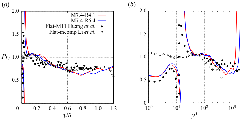
Figure 21. Turbulent Prandtl number at x = 0.85 m as a function of (a) the outer scaling y/\delta and (b) the semi-local wall unit y^* . The DNS results of flat plate hypersonic boundary layers by Huang et al. (2020) and those of incompressible ones by Li et al. (2009) are also included.
