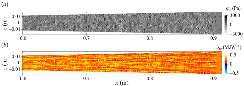
Figure 28. Instantaneous snapshot at the wall for M7.4-R4.1: (a) pressure fluctuation and (b) wall-heat flux.
