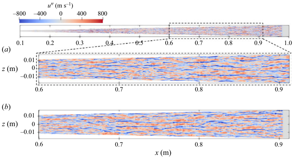
Figure 8. Comparison of velocity fluctuation fields in the wall-parallel planes at y = 0.5 (mm) between (a) the laminar-to-turbulent transition simulation M7.4-LT4.1 and (b) the volumetric rescaling simulation M7.4-R4.1.
