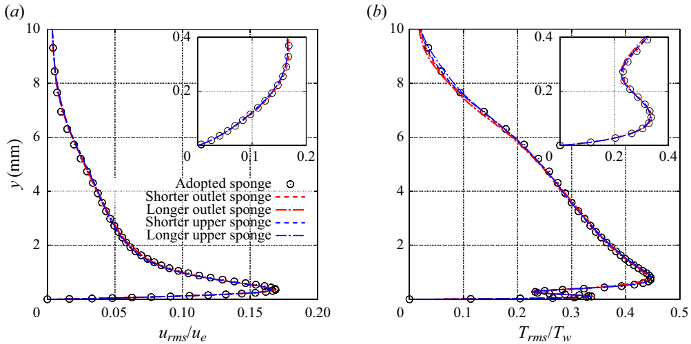
Figure 35. Effects of sponge boundary conditions on fluctuation correlations at x = 0.85 m for (a) streamwise velocity and (b) temperature.
