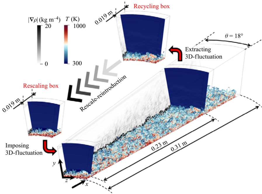
Figure 2. Schematic of the present quasi-spectral viscosity (QSV)-LES of a hypersonic boundary layer over a cone with the volumetric rescaling method. The instantaneous iso-surface of the Q-criterion (second invariant of the velocity gradient tensor) is coloured by temperature. Contours in cross-flow planes show temperature fields in the recycling and rescaling boxes. A contour in a side plane shows the magnitude of the density gradient.
