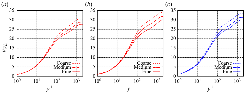
Figure 4. Grid sensitivity study for transformed velocity profiles via Van Driest transformation (van Driest 1951) at x = 0.85 m in (a) M7.4-R4.1, (b) M7.4-R6.4 and (c) M7.4-LT4.1.
