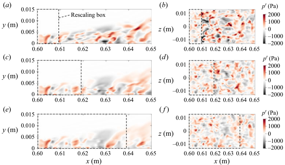
Figure 14. Pressure fluctuation fields around the rescaling box in (a,c,e) the streamwise wall-normal plane at the centre in the azimuthal direction, and (b,d,f) the wall-parallel plane at y = 3.5 mm. Panels show (a,b) short box, (c,d) medium box and (e,f) long box. The rescaling box is surrounded by the black dashed line box.
