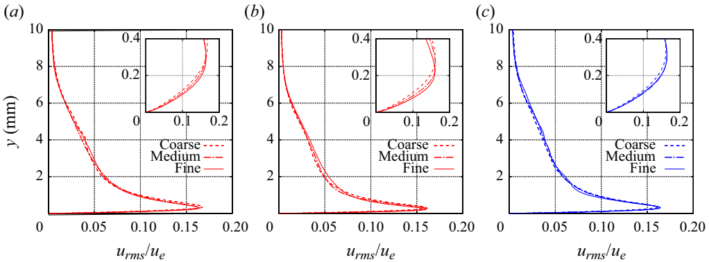
Figure 5. Grid sensitivity study for fluctuation correlations of streamwise velocity at x = 0.85 m in (a) M7.4-R4.1, (b) M7.4-R6.4 and (c) M7.4-LT4.1.
