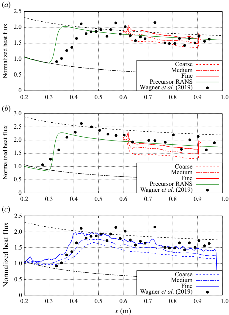
Figure 3. Grid sensitivity study for wall-heat flux in (a) M7.4-R4.1, (b) M7.4-R6.4 and (c) M7.4-LT4.1. The precursor RANS data are included for the rescaling cases. The experiments by Wagner et al. (2019) are also included for all panels. Correlations for the laminar cone boundary layers (Lees 1956) and turbulent ones (White 2006) are given by dash-dotted and dashed lines, respectively.
