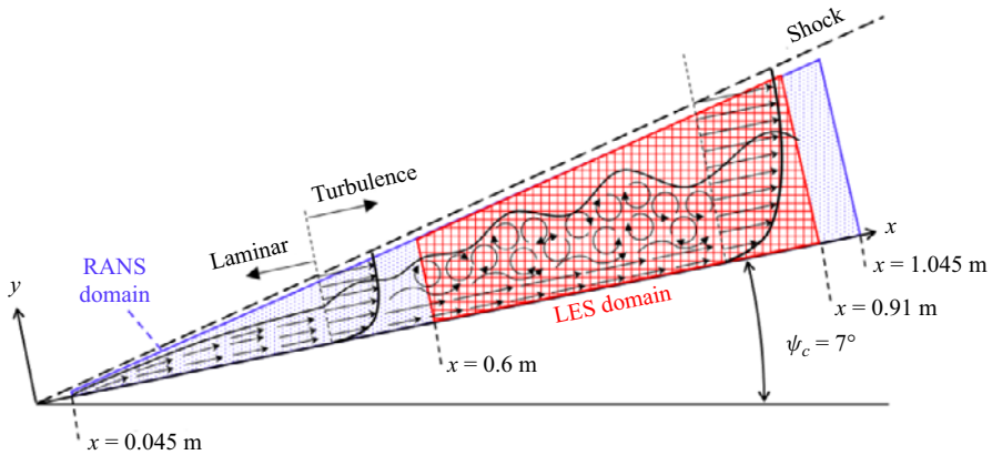
Figure 1. Sketch of the present conical hypersonic boundary-layer configuration.
