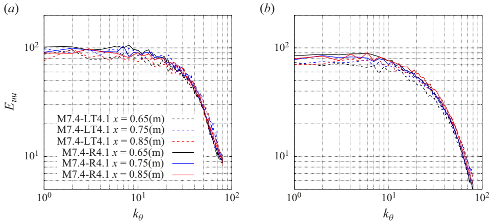
Figure 9. Comparison of one-dimensional spectra of streamwise velocity fluctuations in the azimuthal direction between the laminar-to-turbulent transition simulation M7.4-LT4.1 and the volumetric rescaling simulation M7.4-R4.1 for several x locations. The data are extracted at (a) y^* = 15 and (b) y^* = 300 .
