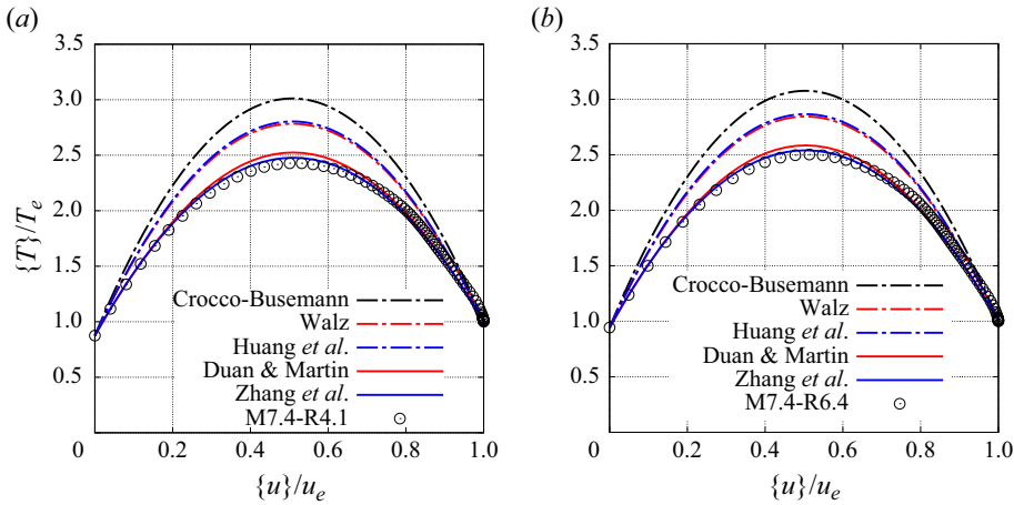
Figure 16. Comparison of temperature–velocity relation at x = 0.85 m between several correlations for (a) M7.4-R4.1 and (b) M7.4-R6.4.
