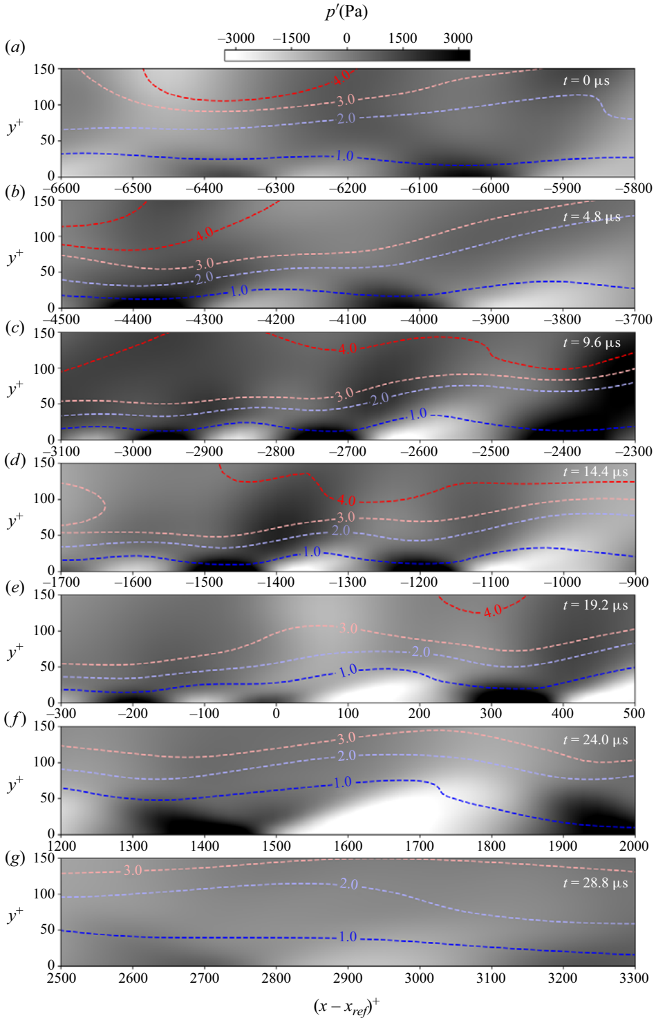
Figure 31. Contours of pressure fluctuations in the (x, y) plane below y^+ = 150 in M7.4-R4.1 at (a) t = 0 \mu\text{s} , (b) t = 4.8 \mu\text{s} , (c) t = 9.6 \mu\text{s} , (d) t = 14.4 \mu\text{s} , (e) t = 19.2 \mu\text{s} , (f) t = 24.0 \mu\text{s} and (g) t = 28.8 \mu\text{s} . Contour lines of local Mach number are given by dashed lines. The visualized regions are selected along the white dash-dotted lines shown in figure 29.
