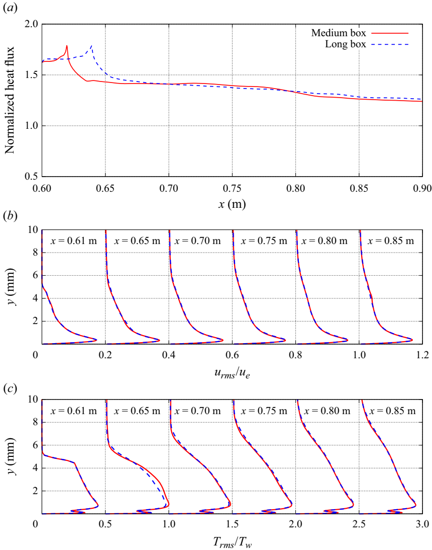
Figure 15. Comparison of (a) wall-heat flux, (b) fluctuation correlations of streamwise velocity and (c) fluctuation correlations of temperature between different rescaling box sizes.
