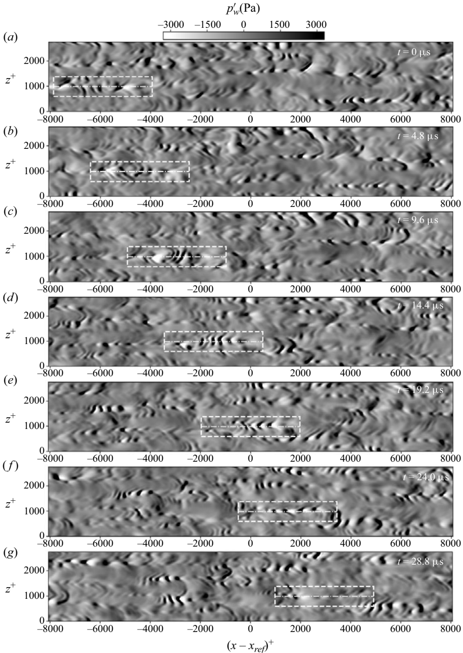
Figure 29. Contours of pressure fluctuations at the wall in M7.4-R4.1 at (a) t = 0 \mu\text{s} , (b) t = 4.8 \mu\text{s} , (c) t = 9.6 \mu\text{s} , (d) t = 14.4 \mu\text{s} , (e) t = 19.2 \mu\text{s} , (f) t = 24.0 \mu\text{s} and (g) t = 28.8 \mu\text{s} . A selected series of trapped waves is surrounded by the white dashed line square box at each t to explore its propagation. Profiles of pressure fluctuations along the white dash-dotted lines are extracted and shown in figure 30 .
