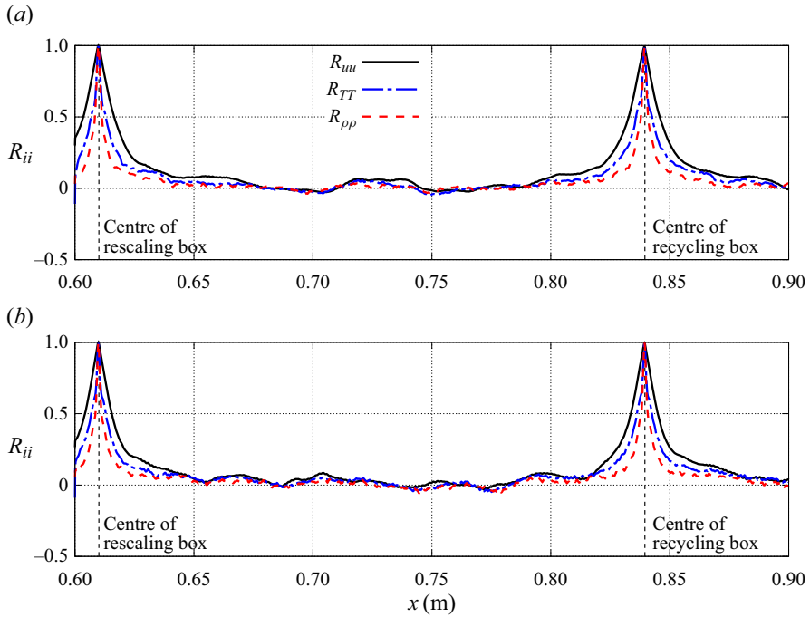
Figure 34. Two-point correlations of streamwise velocity, temperature and density components for the centre of the rescaling box in the streamwise direction. The data are obtained at y^* = 10 for (a) M7.4-R4.1 and (b) M7.4-R6.4.
