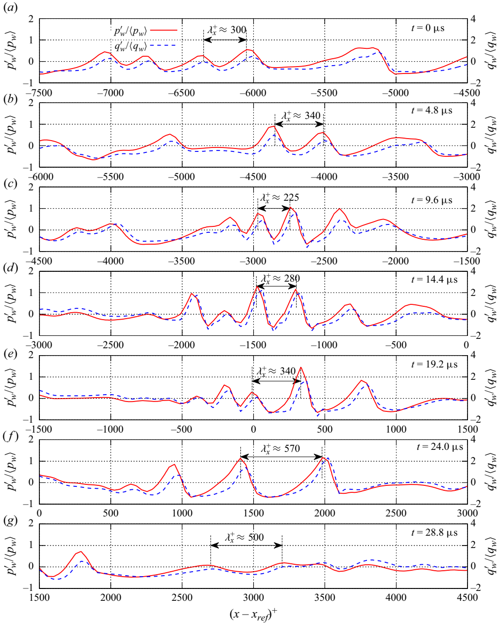
Figure 30. Profiles of pressure and wall-heat flux fluctuations at the wall along the white dashed-dotted lines in figure 29 at (a) t = 0 \mu s , (b) t = 4.8 \mu s , (c) t = 9.6 \mu s , (d) t = 14.4 \mu s , (e) t = 19.2 \mu s , (f) t = 24.0 \mu s and (g) t = 28.8 \mu s .
