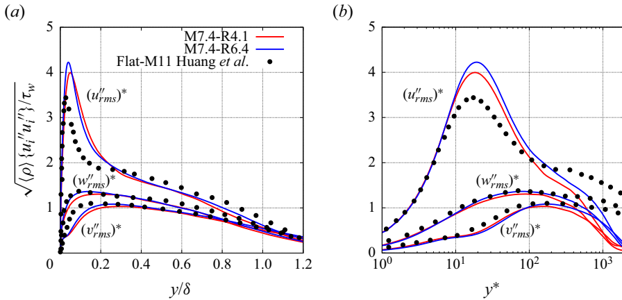
Figure 17. Velocity fluctuation correlations at x = 0.85 m as a function of (a) the outer scaling y/\delta and (b) the semi-local wall unit y^* . The DNS results of flat plate hypersonic boundary layers by Huang et al. (2020) are also included.
