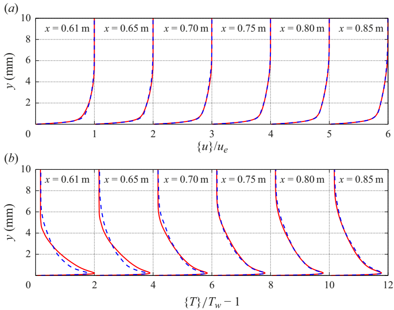
Figure 11. Mean profiles of (a) velocity and (b) temperature for Re_m = 4.1 \times 10^6 \text{ m}^{-1} cases. Results of the volumetric rescaling simulation M7.4-R4.1 (red solid line) are compared with those of the laminar-to-turbulent transition simulation M7.4-LT4.1 (blue dashed line).
