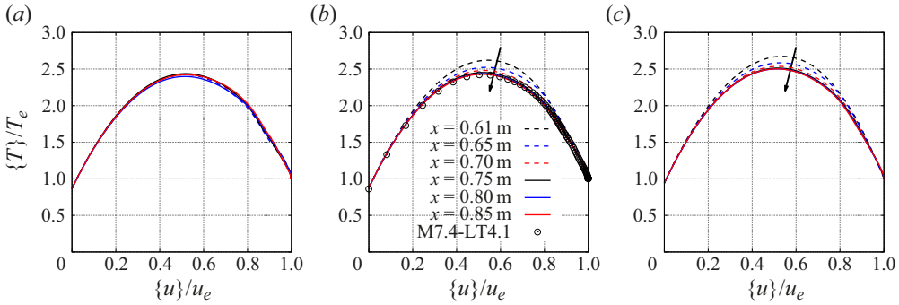
Figure 13. Temperature–velocity relation for (a) M7.4-LT4.1, (b) M7.4-R4.1 and (c) M7.4-R6.4 at several x locations. Black circles in (b) represent the M7.4-LT4.1 data at x = 0.85 m.
