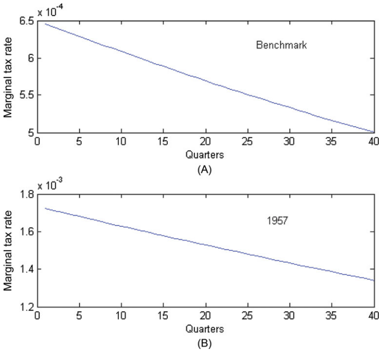
FIGURE 1. Dynamic path of the marginal tax rate. The two panels show the absolute deviations of \tau from steady state values after a one-unit standard deviation in z .
