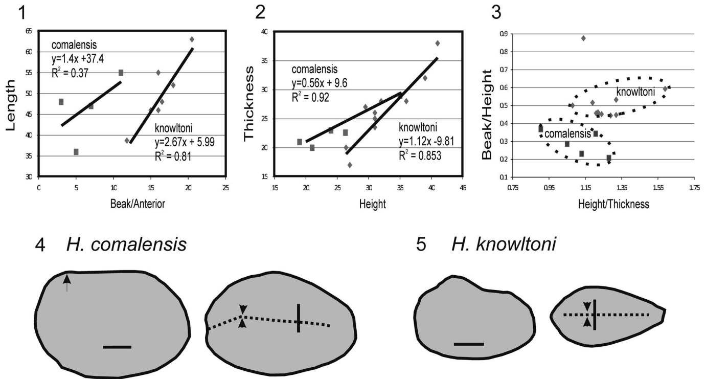
Figure 8. Comparisons of H. comalensis with H. knowltoni . (1) Distance of umbo from anterior margin versus valve length in millimeters. (2) Cross plot of valve height to thickness. (3) Cross plot of ratio of height to thickness versus ratio of umbo distance to height. The area of H. comalensis is separate from that of H. knowltoni . The outlier specimen is from the Comanche Peak Formation NPL44903. (4) Left lateral and dorsal outlines of H. comalensis illustrated by Whitney (1937, pl. 13, figs. 3, 4). (5) Left lateral and dorsal outlines of H. knowltoni holotype USNM145644. Scale bars = 1 cm; dashed line marks the commissure; arrows indicate beaks.
