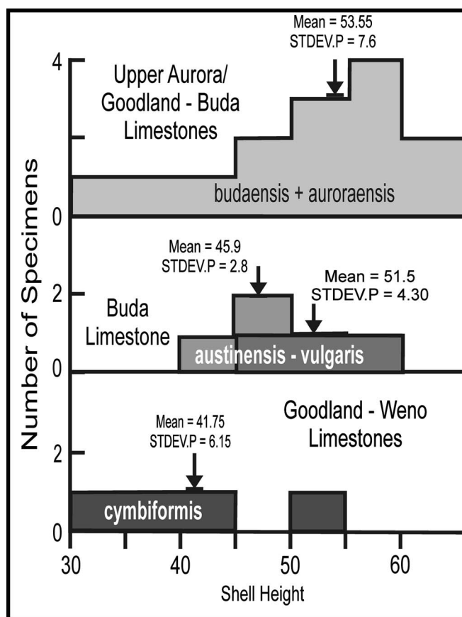
Figure 6. Histograms show the difference in shell height of five cylindrical homomyid species in stratigraphic succession. STDEV.P is Excel standard deviation function.
