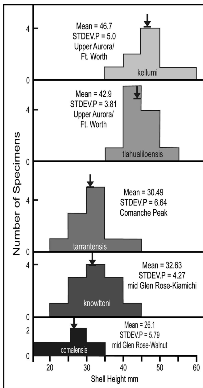
Figure 5. Histograms show the difference in shell height of five streamlined homomyid species in stratigraphic succession. STDEV.P is Excel standard deviation function.
