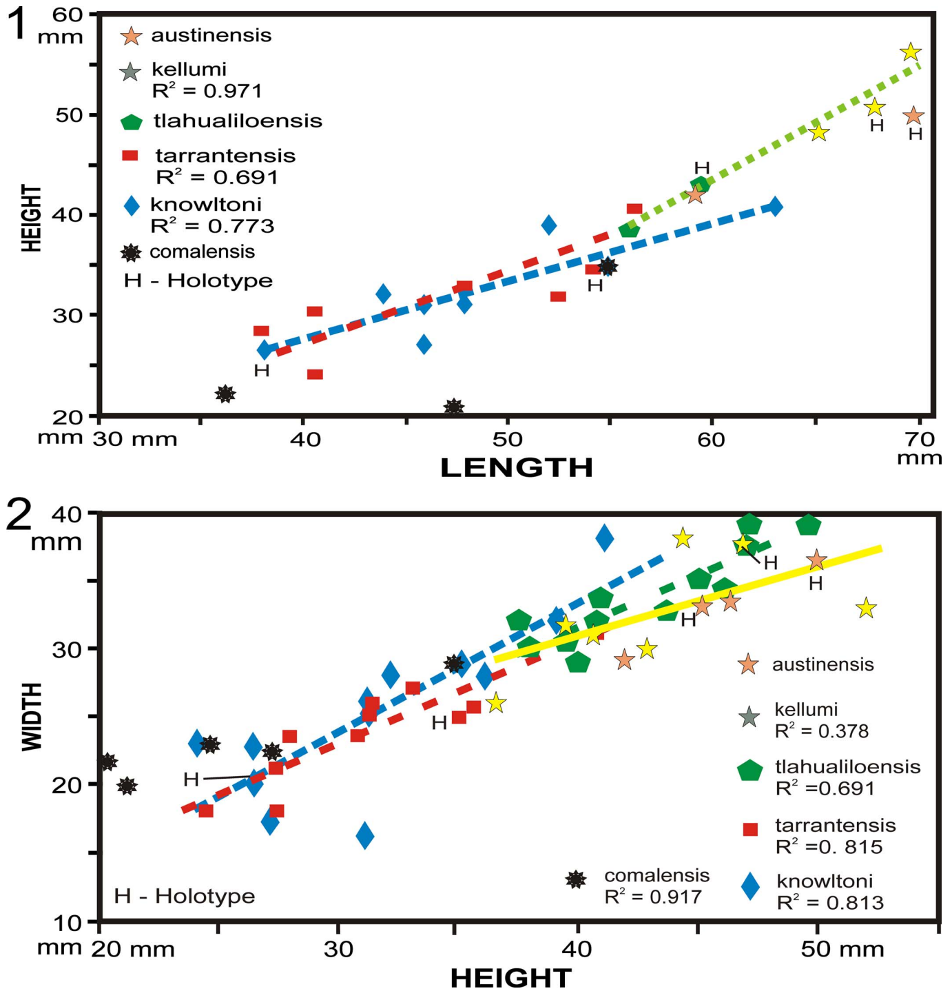
Figure 7. Cross plots of H. knowltoni , H. comalensis , and H. kellumi and their synonyms. (1) Length to height; (2) height to width.
