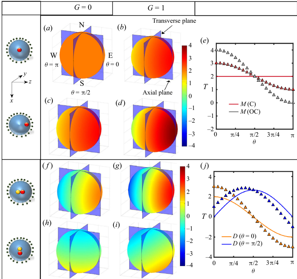
Figure 4. Temperature ( T ) contours on the droplet surface for two ambient thermal gradients G = 0 and 1. Droplets with (a–d) monopole-based, and (f–i) dipole-based thermal singularities. On the droplet surface, the \theta direction begins at east (E) and ends at north (N) in the clockwise direction covering south (S) and west (W) points. The droplet is subjected to ambient flow experienced as downstream at \theta = 0 and upstream at \theta = \pi . (e,j) Temperature profiles in the \theta direction for fixed \phi = 0 . Continuous lines for G = 0 , and triangles for G = 1 . Red for centred (C) monopole, grey for off-centred (OC) monopole, orange for dipole oriented in the streamwise direction, and blue for dipole oriented in the cross-stream direction. Parameters are S = 2 , \kappa = 1 . Note that the temperature profiles are independent of other parameters such as droplet offset location from the axis b , Pe_s , \mu , Ma_T , Ma_\Gamma and others.
