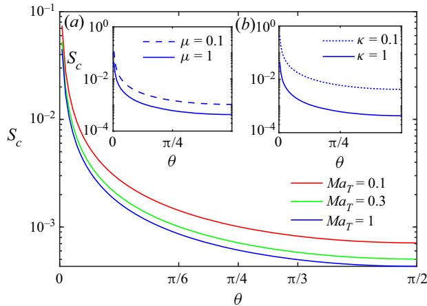
Figure 7. Critical dipole strength S_c as a function of dipole orientation angle \theta for Ma_T = 0.1 (red), Ma_T = 0.3 (green), and Ma_T = 1 (blue). Parameters are Pe_s = 0.1 , G = 1 , Ma_T = 10 , \kappa = 1 , \mu = 1 , R_0 = 5 and Bo = 0 . Insets for different (a) viscosity and (b) thermal conductivity.
