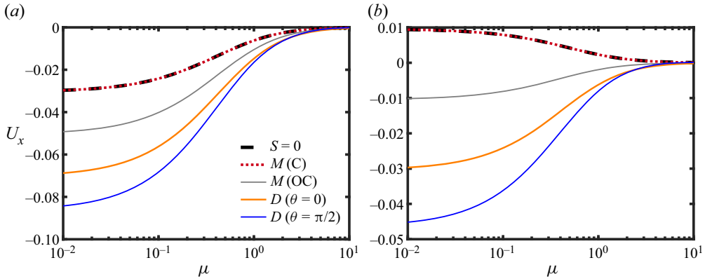
Figure 15. Droplet cross-stream migration velocity U_x versus viscosity ratio \mu for S = 0 (dashed line), centred monopole (dotted line), off-centred monopole (grey), dipole oriented streamwise (orange) and dipole oriented transversely (blue), for (a) G = 1 , \omega = 1 , and (b) G = -1 , \omega = 1 . Other parameters are S = 2 , Ma_T = 1 , Ma_\Gamma = 10 , Pe_s = 0.1 , \kappa = 1 , b = 1 , R_0 = 5 and Bo/Ca = 1 .
