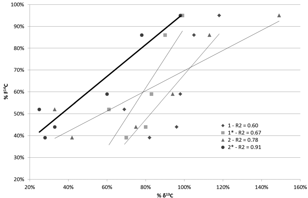
Figure 2 % exchange F^{14}C versus % exchange \delta^{13}C excluding coal fire
