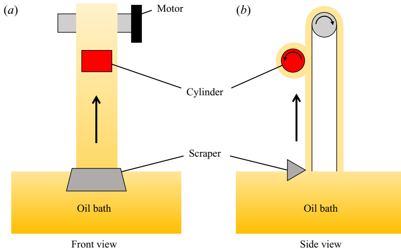
Figure 1. Schematic diagram of the experimental apparatus showing a cylinder balanced on the belt, which is covered in a layer of oil. Videos of this experiment are provided as supplementary material (Movies 1 and 2) available at https://doi.org/10.1017/jfm.2021.284 .
