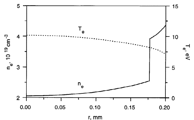
Fig. 13. Radial distribution of electron density n_e and electron temperature T_e at moment t = 100 ns, for the same parameters as in Figure 11.
