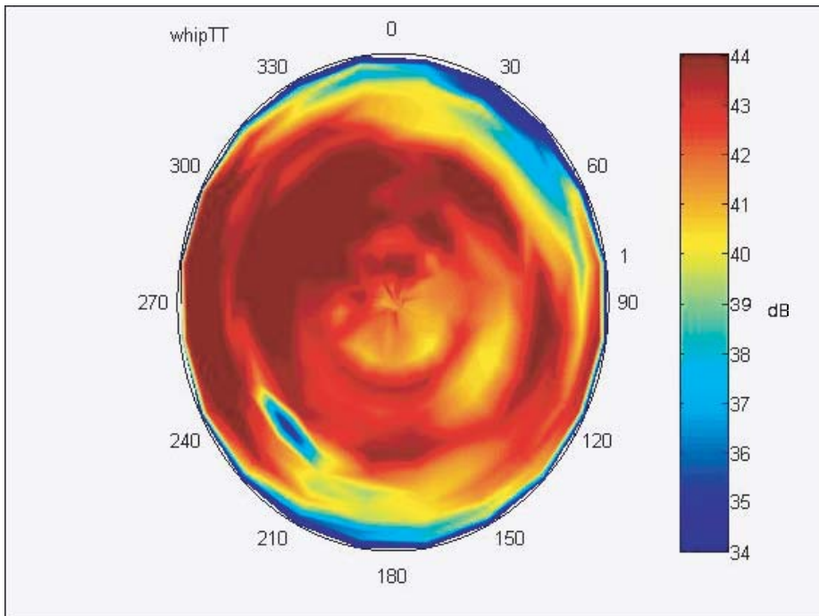
Figure 7. Whip antenna at 30° elevation.
