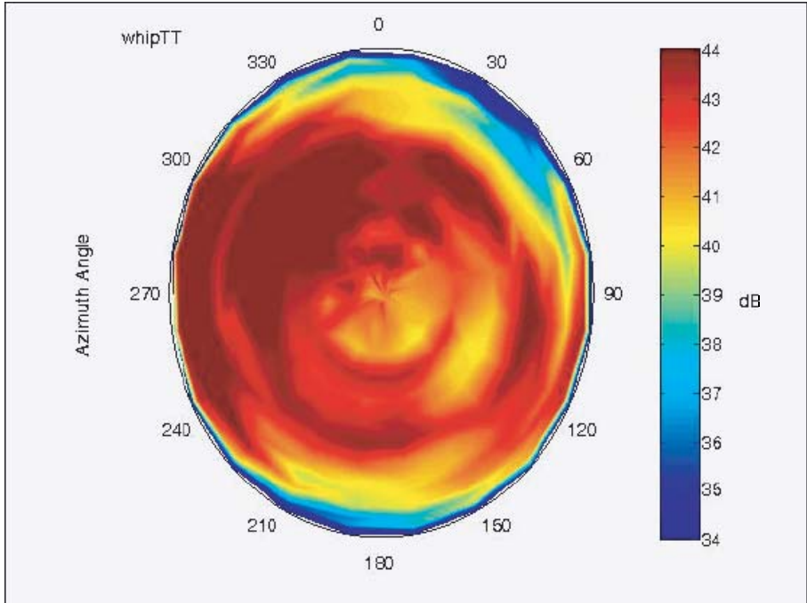
Figure 6. Gain pattern for horizontal whip antenna.
