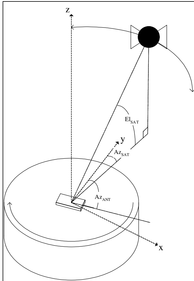
Figure 4. Hardware Setup.
