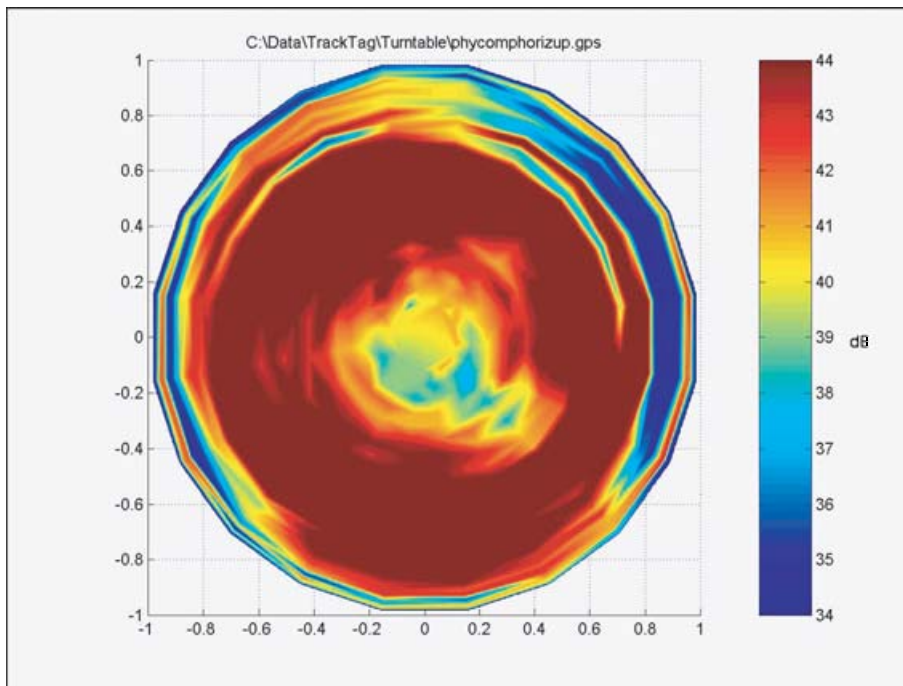
Figure 9. Ceramic chip antenna pointing upwards.
