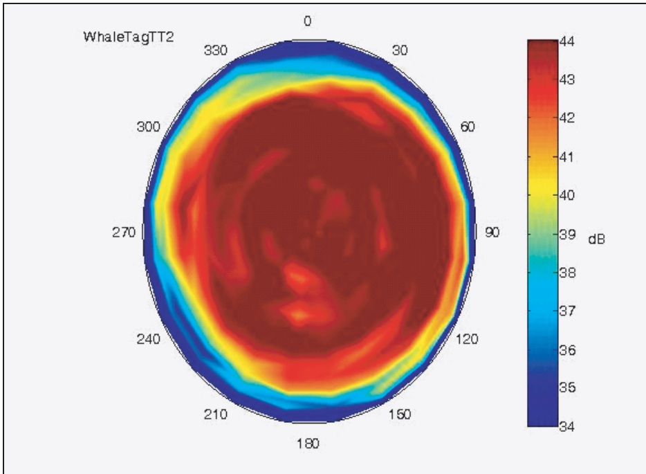
Figure 8. Gain pattern for horizontal patch antenna.
