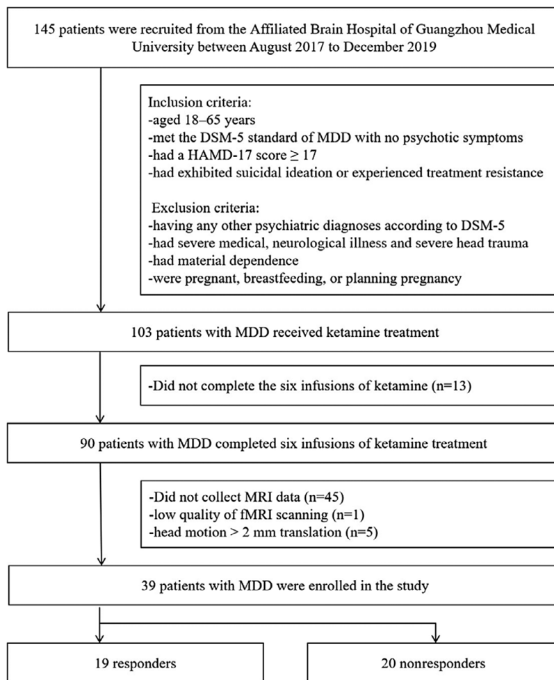
Figure 1. Flowchart. DSM-5, diagnostic and statistical manual of mental diseases-5; fMRI, functional magnetic resonance imaging; HAM-D-17, 17-item Hamilton Depression Scale; MDD, major depressive disorder; MRI, magnetic resonance imaging.
