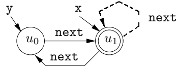
Effect of x.\text{next} = y on Figure 8:
