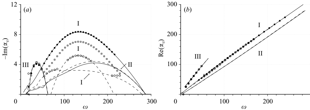
FIGURE 15. (a) Spatial amplification rates and (b) wavenumbers in the \check{x} = x_v direction ( \check{\varphi} = \varphi_v = 45.86^\circ ) from SLST (lines) and from adapted DNS (case Adapted-vortex-oriented , symbols) as functions of the frequency. The primary states for the SLST and the three-dimensional base flows for the DNS have been defined according to the w_v -fixed approach (solid lines, dots), the v_v -fixed approach (dashed lines, circles) and to the v_v - w_v -fixed approach (only DNS, squares).
