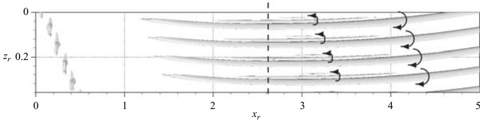
FIGURE 4. Visualization of vortical structures ( \lambda_2 -isosurfaces, \lambda_2 = -5 ) for the steady fundamental case ( x_{0,r} = 1.5 , z_{0,r} = 0.09 , \varphi_r = 45.86^\circ ). Arrows indicate the rotation direction of the vortices. The dashed line shows the position of the crosscut plane of figure 5.
