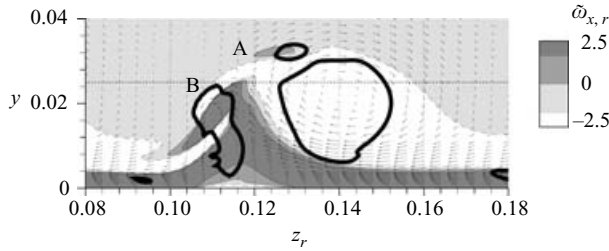
FIGURE 24. Visualization over the section plane x_r = 3.57 of figure 22: [\tilde{w}_r, \tilde{v}_r] -vectors; \tilde{\omega}_{x,r} -isocontours (shaded); \lambda_2 -isocontours (thick lines, \lambda_2 = -10 ). The horizontal dotted line denotes the undisturbed boundary-layer thickness.
