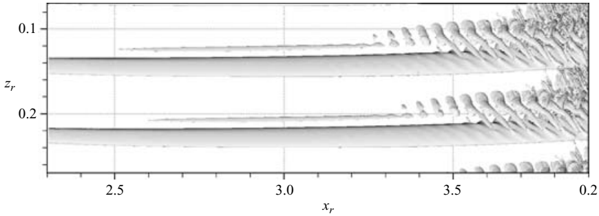
FIGURE 22. Visualization of vortical structures ( \lambda_2 -isosurfaces, \lambda_2 = -10 ) for case Steady + \omega 120 : x_{0,r} = 1.5 , z_{0,r} = 0.10 , \varphi_r = 45.86^\circ .
