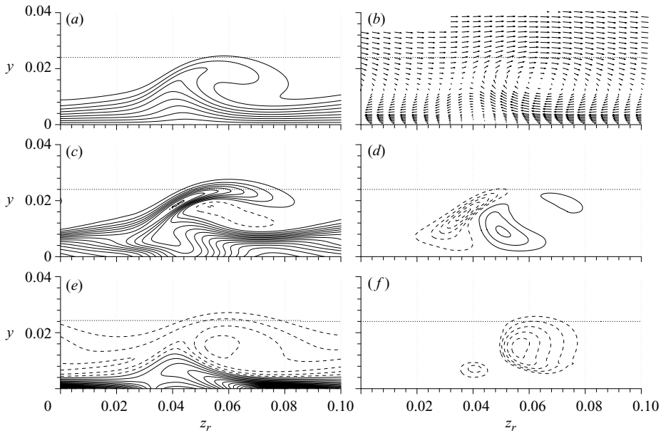
FIGURE 5. Flow field in the crosscut plane x_r = 2.61 of figure 4 ( x \approx 3.32 ): (a) \tilde{u}_r -isocontours, \Delta = 0.1 ; (b) [\tilde{u}_r, \tilde{v}_r] -vectors; (c) \partial \tilde{u}_r / \partial y -isocontours, \Delta = 10.0 ; (d) (\partial u_r / \partial z_r) / u_{b,s,e} -isocontours, \Delta = 10.0 ; (e) \tilde{\omega}_{x,r} -isocontours, \Delta = 2.5 ; (f) \lambda_2 -isocontours, \Delta = 5.0 . Dashed lines correspond to negative values. The horizontal dotted line denotes the undisturbed boundary-layer thickness \delta_s in z_r = 0 . The variation of \delta_s over the considered z_r -interval is less than 1%.
