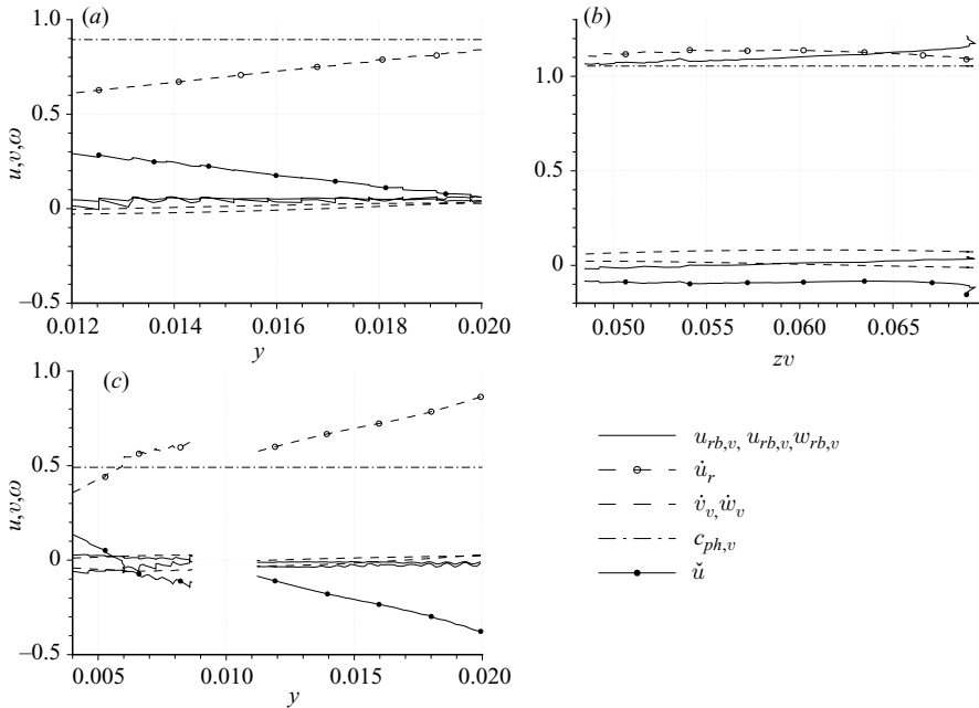
FIGURE 37. Primary-state velocity components and rigid-body velocity components (right-hand side of (8.1)) at points of the vortex cores from figure 32. The function \check{u} is computed imposing the x_v -component of (8.1) for type I and type III modes, and the z_v -component for the type II mode. The component of the rigid-body velocity directly determined by (8.1) is not plotted. The variable on the abscissa is different in different figures. (a) Type I, \text{Re}(\alpha_v) = 134 , c_{ph,v} = 0.89 ; (b) type II, \text{Re}(\alpha_v) = 162 , c_{ph,v} = 1.05 ; (c) type III, \text{Re}(\alpha_v) = 62 , c_{ph,v} = 0.49 .
