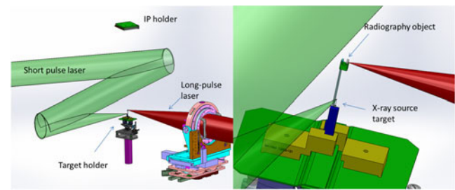
Figure 1. Radiography setup with imaging plate, target holder and laser beams. On the right a magnification of the target holder with x-ray source and radiography sample.
