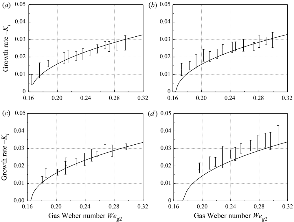
Figure 20. Growth rate of solutions at different concentrations. (a) Deionized water: U_l = 1.820 \text{ m s}^{-1} , Re_l = 378.4 , \rho = 0.0012 , \Omega_{s2} = 0.0980 ; (b) 20 % glycerol aqueous solution: U_l = 1.779 \text{ m s}^{-1} , Re_l = 211.8 , \rho = 0.00114 , \Omega_{s2} = 0.1005 ; (c) 40 % glycerol aqueous solution: U_l = 1.704 \text{ m s}^{-1} , Re_l = 93.7 , \rho = 0.00109 , \Omega_{s2} = 0.1049 ; (d) 60 % glycerol aqueous solution: U_l = 1.635 \text{ m s}^{-1} , Re_l = 31.6 , \rho = 0.00104 , \Omega_{s2} = 0.1093 . (Full line is theoretical curves; error bars are measured results; gas is air; \rho_g = 1.2 \text{ kg m}^{-3} , a = 0.0002 \text{ m} , f_s = 142 \text{ Hz} ).
