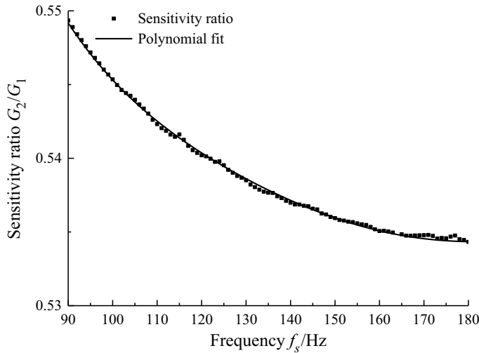
Figure 7. Ratio of microphone sensitivities.
