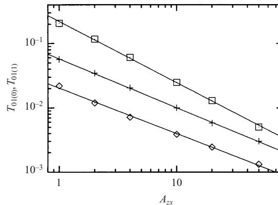
FIGURE 5. Value of T_{01(0)} (regime I) or T_{01(1)} (regimes II and III) vs. A_{zx} for A_{zx} \geq 1 , Ra_z = 50\,000 and Bi = 0.1 ( \diamond ), Bi = 2 ( + ), Bi = 1000 ( \square ). The following power-laws are observed: T_{01(0)} \propto A_{zx}^{-0.71} (regime I), T_{01(1)} \propto A_{zx}^{-0.76} (regime II) and T_{01(1)} \propto A_{zx}^{-0.95} (regime III). Best-fit lines through the data are shown.
