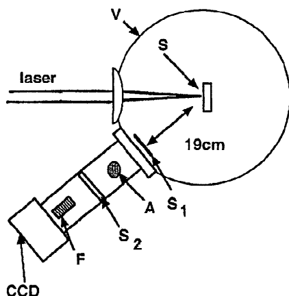
Fig. 1. Schematic of the experimental setup. V: vacuum chamber, S: solid target, S1: external slit ( 100 \mu\text{m} width), A: gold coated spherical mirror, S2: Slit 300 (\mu\text{m}) width, F: flat field grating (1200 lines/mm), and CCD: Black illumination type CCD camera.
