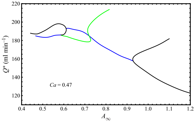
Figure 9. The dimensional flow rates, Q^* , corresponding to the computed steadily propagating solutions shown in figure 8 as a function of the initial level of collapse A_\infty . All solutions correspond to a fixed capillary number of Ca = 0.47 . The colour coding for the solution branches is the same as in figure 8.
