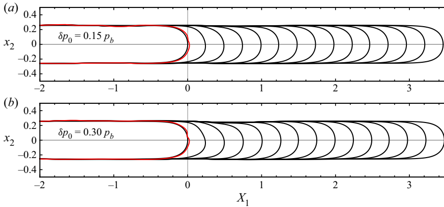
Figure 10. Finger propagation in a stationary (laboratory) frame of reference for an initially uncollapsed channel, A_\infty = 1 . Unsteady numerical simulations were initialised with a steady solution at Ca = 0.47 . The time increment between the interfaces is \delta t = 0.2 . During the time evolution, the interface is subject to a transient local pressure perturbation in the form of (3.1). The amplitude of the perturbation is (a) \delta p_0 = 0.15 p_b and (b) \delta p_0 = 0.30 p_b . The interfaces at the time t_p are highlighted in red. The deformation on the interface quickly decays and a steadily propagating symmetric finger is established.
