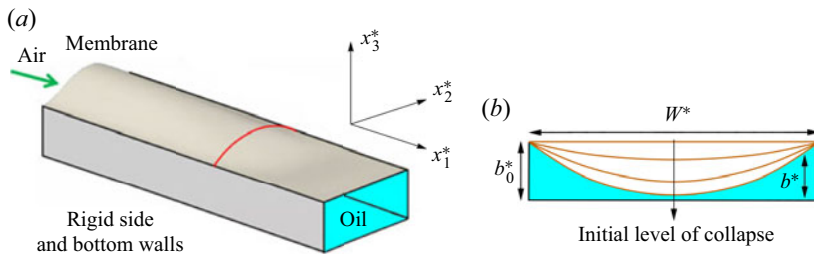
Figure 1. The elasto-rigid channel consists of two rigid sidewalls, a rigid lower wall and a deformable upper wall. The cross-section of the channel has width W^* and undeformed height b_0^* . The height of the deformed sheet is b^*(x_1^*, x_2^*) . An air finger propagates into the fluid-filled channel along the x_1^* direction.
