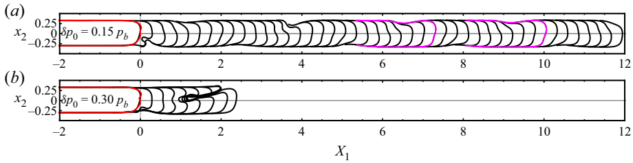
Figure 12. Finger propagation in a stationary (laboratory) frame of reference for a moderately collapsed channel, A_\infty = 0.8 . Unsteady numerical simulations were initialised with a steady solution at Ca = 0.47 . The time increment between the interfaces is \delta t = 0.27 . During the time evolution, the interface is subject to a transient local pressure perturbation in the form of (3.1). The amplitude of the perturbation is \delta p_0 = 0.15 p_b (a) and \delta p_0 = 0.30 p_b (b). The interfaces at the time t_p are highlighted in red and the deformation on the interface is advected to the narrower side of the asymmetric finger and decreases in amplitude. In (a), the finger tip rapidly develops an oscillatory motion. The first and last interfacial positions of one oscillation are highlighted in pink. The period and wavelength of the oscillation are T = 2.7 and L = 2.7 channel widths, respectively. In order to aid the visualisation of the oscillations, we are only plotting the interfaces for 1.5 channel widths behind the finger tip. In (b), the interface develops a deep cleft and we terminate the simulation when the sides of the cleft intersect.
