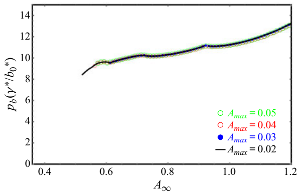
Figure 18. Finger pressure at Ca = 0.47 as a function of the initial level of collapse for different mesh resolutions. The results are indistinguishable for A_{max} \leq 0.03 .
