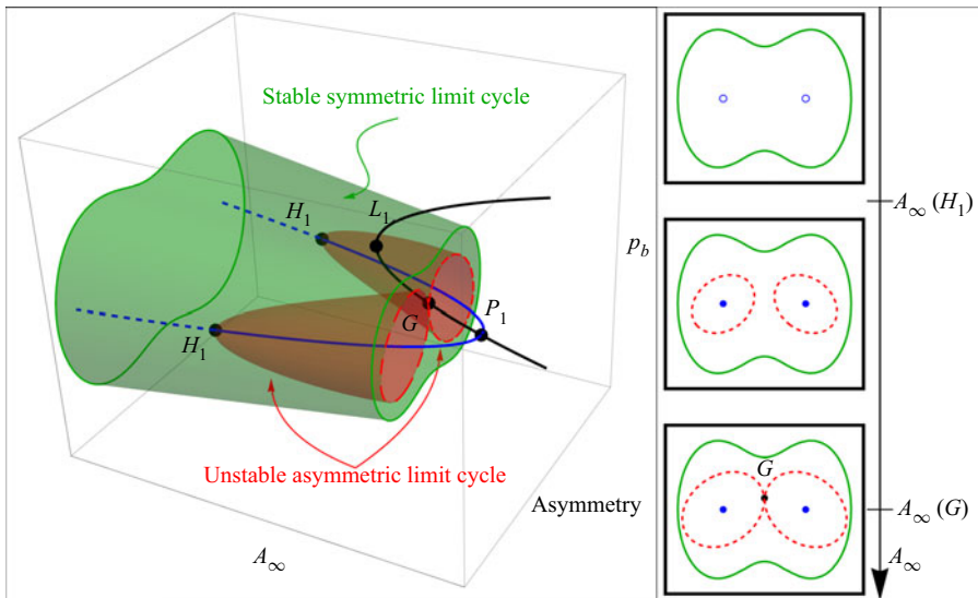
Figure 14. A sketch of the proposed bifurcation scenario in the region 0.9 < A_\infty < 0.95 at fixed Ca = 0.47 . A symmetric steadily propagating finger state (black line) undergoes a symmetry-breaking pitchfork bifurcation at A_\infty = 0.93 followed by a limit point at A_\infty = 0.927 . The two steadily propagating asymmetric states that arise from the pitchfork bifurcation (blue line) each undergo a subcritical Hopf bifurcation at A_\infty = 0.912 . Two unstable limit cycles emanate from the Hopf bifurcation on each asymmetric branch for A_\infty > 0.912 . We conjecture that these unstable limit cycles become a symmetric limit cycle via a gluing bifurcation on the symmetric branch in the region between the limit point and the pitchfork bifurcation, 0.927 > A_\infty > 0.93 . The symmetric limit cycle is likely to be stabilised through a limit point (not shown).
