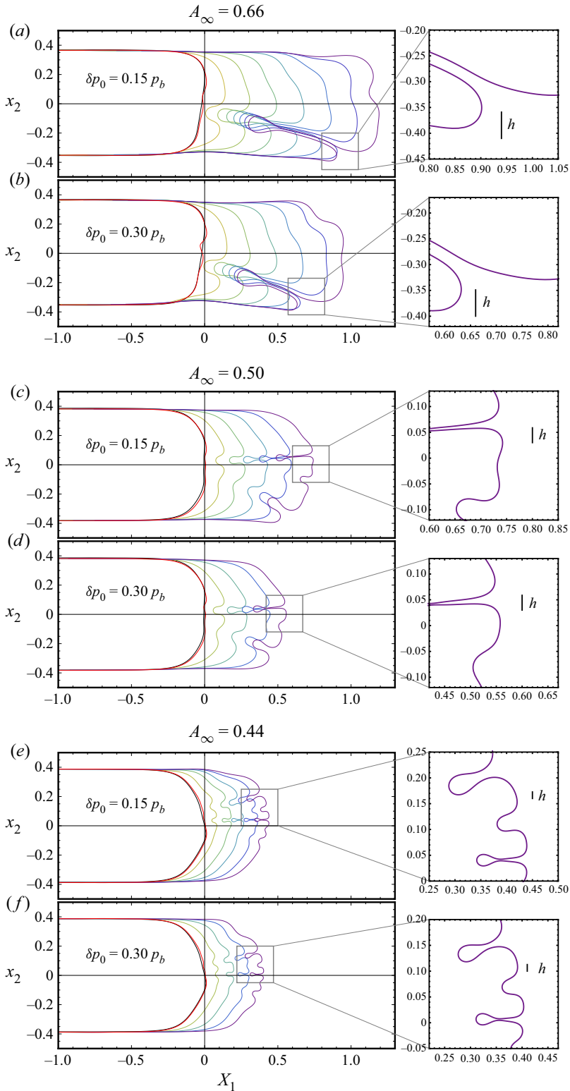
Figure 13. For caption see next page.
