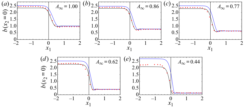
Figure 16. Membrane height along the centreline of the channel ( x_2 = 0 ) for decreasing values of A_\infty . The red circles indicate the experiments of Ducloué et al. (2017b), while solid lines indicate steady numerical solutions of the fully coupled fluid–structure interaction problem in the presence (black) and absence (blue) of the liquid films on the upper and lower walls. The tip of the air finger is located at x_1 = 0 .
