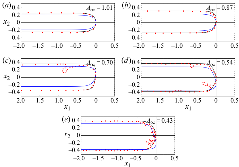
Figure 15. Finger shapes for decreasing values of A_\infty . The red circles indicate the experiments of Ducloué et al. (2017b), while solid lines show steady numerical solutions of the fully coupled fluid–structure interaction problem in the presence (black) and absence (blue) of the liquid films on the upper and lower walls. The experimental fingers shown in (c–e) are snapshots of unsteady modes of propagation where small-scale fingers are continually formed near the tip and advected around the curved front.
