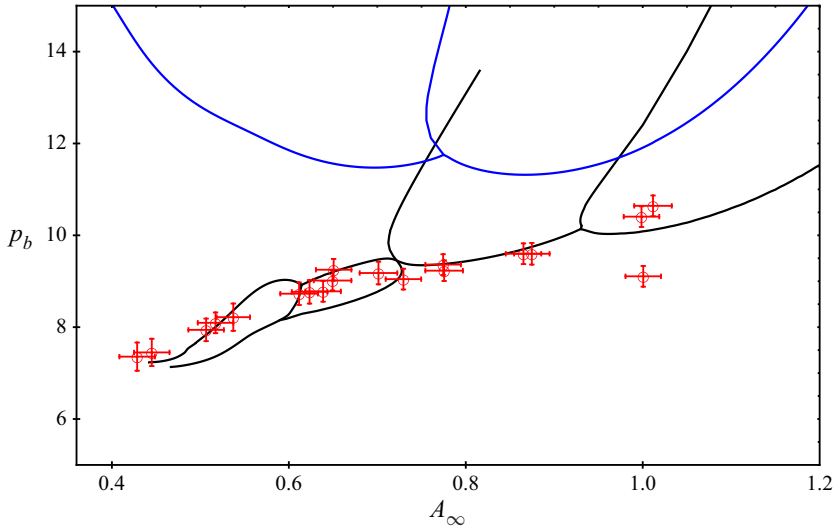
Figure 7. Finger pressure p_b = p_b^*/(\gamma^*/b_0^*) on the capillary scale as a function of the initial level of collapse A_\infty for a fixed capillary number of Ca = 0.47 . The experimental data from Ducloué et al. (2017b) are shown with red circles and the error bars correspond to the standard deviations of three experiments. The black lines show steady solutions of the model, and blue lines are the corresponding solutions without any liquid-film corrections.
