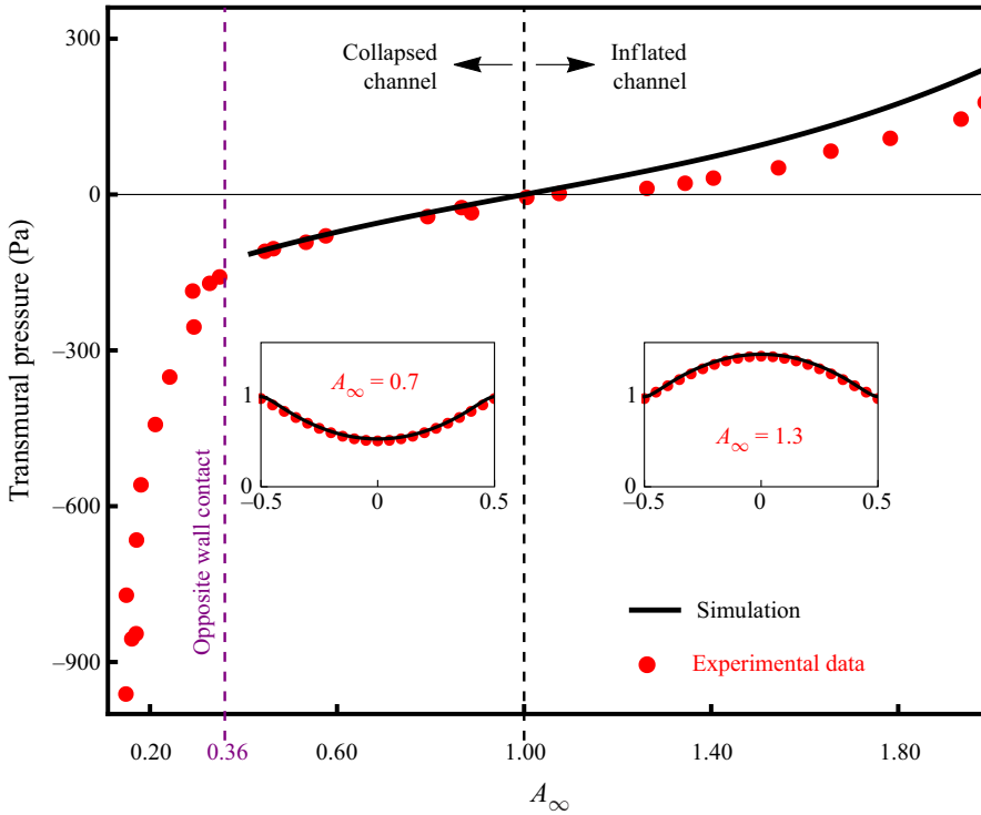
Figure 4. Variation of the transmural pressure as a function of the level of collapse, which provides a constitutive relation for the channel (the channel law). The red circles indicate the experiments of Ducloué et al. (2017b), while the black line is the numerical solution of the Föppl-von Kármán equation (2.3a,b) for experimental parameters and a pre-stress \sigma_{22}^{(0)*} = 30 kPa and A_\infty > 0.36 , the point of near-opposite wall contact.
