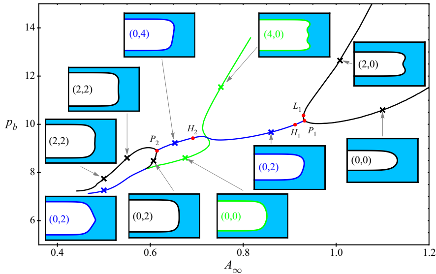
Figure 8. Steady numerical solutions with liquid-film corrections shown in terms of the variation of the finger pressure p_b as a function of the initial level of collapse A_\infty , for a fixed capillary number of Ca = 0.47 . The results are similar to those shown in figure 7, but here, each solution branch is shown with a different colour and the finger morphologies for different parameter values are illustrated with inset images. Solutions that are symmetric about the channel's centreline are represented as black or green lines; asymmetric solutions are shown as blue lines; P_1 and P_2 denote pitchfork bifurcations, H_1 and H_2 the locus of Hopf bifurcations and L_1 is a limit point. The number of positive eigenvalues are indicated by the pair of numbers in the inset images, where the first number counts the real positive eigenvalues and the second one the number of complex eigenvalues with positive real part; these occur in complex conjugate pairs.
