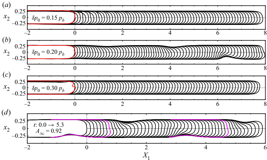
Figure 11. Finger propagation in a stationary (laboratory) frame of reference for an initially slightly collapsed channel, A_\infty = 0.92 and fixed flow rate. Unsteady numerical simulations were initialised with a steady solution at Ca = 0.47 . The time increment between the interfaces is \delta t = 0.1 . During the time evolution, the interface is subject to a transient local pressure perturbation given by (3.1). The amplitude of the perturbation is (a) \delta p_0 = 0.10 p_b ; (b) \delta p_0 = 0.20 p_b and (c) \delta p_0 = 0.30 p_b . The interfaces at the time t_p are highlighted in red. For the smallest-amplitude perturbation the interface quickly returns to the linearly stable steadily propagating asymmetric state. For the intermediate-amplitude perturbation the finger evolves towards a periodic solution, shown in (d). The first and last interfacial positions of one complete oscillation are highlighted in pink and the period T = 3.5 . For the largest-amplitude perturbation, the finger evolves towards the alternative steadily propagating asymmetric state, in which the asymmetric finger has been reflected about the channel's centreline.
