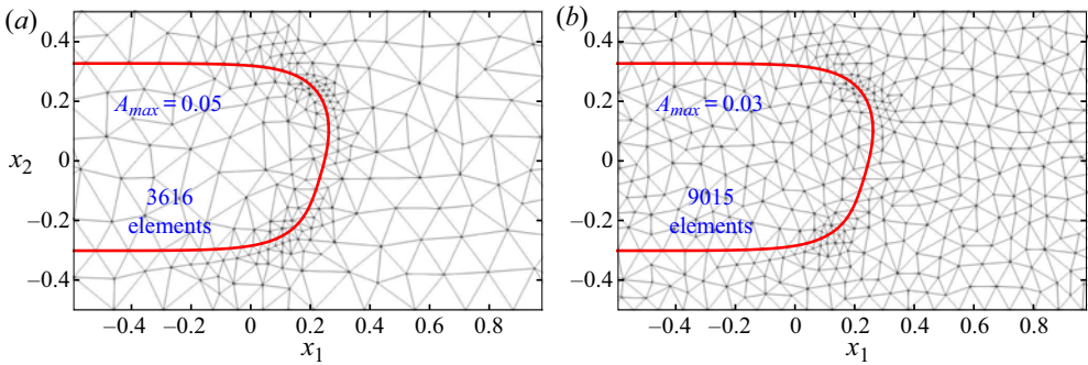
Figure 17. Steadily propagating asymmetric fingers for A_\infty = 0.8 , Ca = 0.47 at two different mesh resolutions (a) A_{max} = 0.05 , (b) A_{max} = 0.03 .
