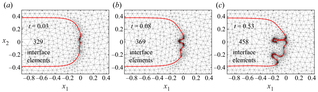
Figure 3. Time evolution of interface at Ca = 0.47 and A_\infty = 0.5 illustrating the remeshing as the interface morphology changes. The snapshots are taken from the simulation shown in figure 13(d) .
