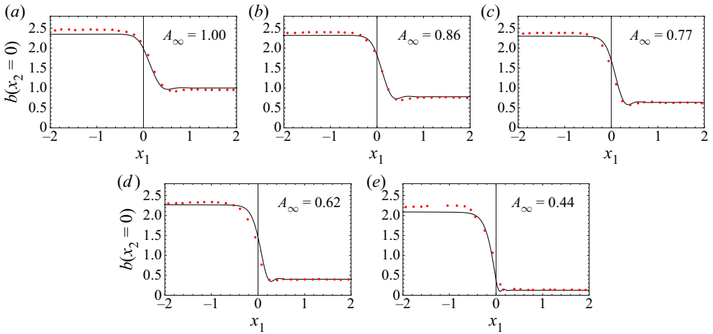
Figure 5. Membrane height along the centreline of the channel ( x_2 = 0 ) for decreasing values of A_\infty . The red circles indicate the experiments of Ducloué et al. (2017b), while black lines indicate steady numerical solutions of the fully coupled fluid–structure interaction model. The tip of the air finger is located at x_1 = 0 .
