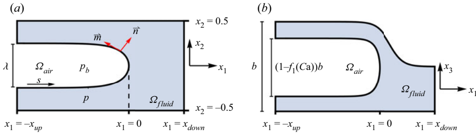
Figure 2. (a) Numerical domain in the frame of reference moving with the finger tip: x_2 = -0.5 and x_2 = 0.5 are the rigid sidewalls; x_1 = -x_{up} is the upstream end of the domain and x_1 = x_{down} is the downstream end of the domain. (b) Sketch of the thin layers of viscous fluid left behind of the advancing interface, at x_2 = 0 . The total thickness of the film layers is f_1(Ca)b . The thickness of the air finger is (1 - f_1(Ca))b .
