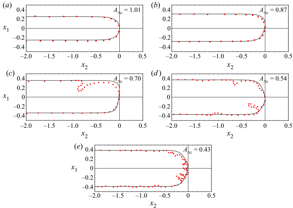
Figure 6. Finger shapes delimited by the air–liquid interface for decreasing values for A_\infty . The red circles indicate the experiments of Ducloué et al. (2017b), while black lines show steady numerical solutions of the fully coupled fluid–structure interaction model. The experimental fingers shown in (c–e) are snapshots of unsteady modes of propagation where small-scale fingers are continually formed near the tip and advected around the curved front.
