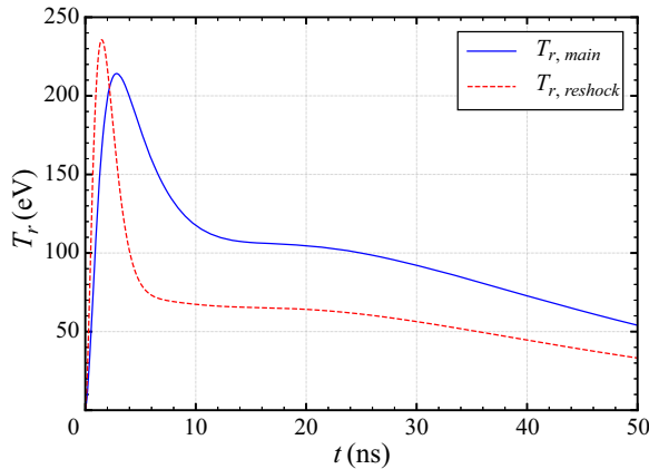
Figure 3. Radiation temperature sources, applied to the x = 0 and x = W boundaries. The sources are defined by (3.23) and the coefficients in table 8.
