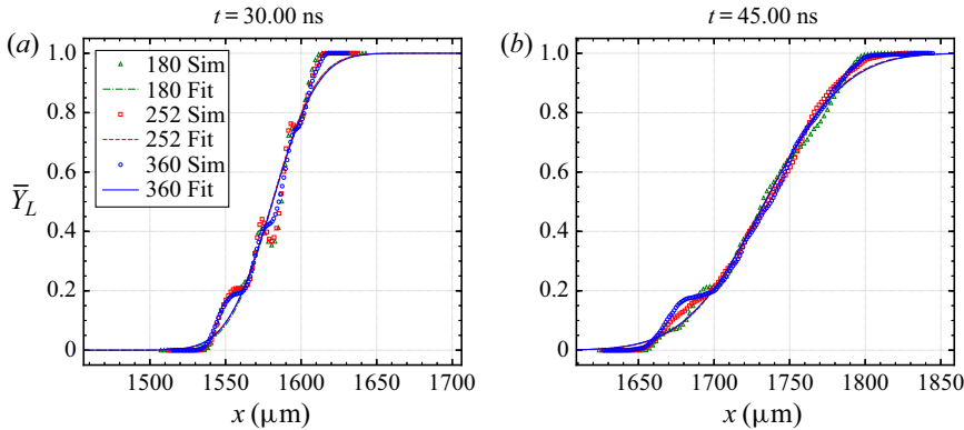
Figure 9. Instantaneous profiles of the Reynolds-averaged mass fraction \bar{Y}_L of the light material M_L versus axial distance at two times in the baseline simulations. Symbols indicate data extracted directly from the simulations (Sim). The data are under-sampled for clarity in the figure, i.e. for each case, there are more data available than there are symbols drawn. Lines indicate fits (Fit) to the simulation data using the analytic form (4.3). The abscissa limits are chosen such that the centre of each plot is x = x_c , as defined in the text, and the abscissa range is 250 \mu\text{m} . The legends state \mathcal{N}_{y,z,2} as defined in the caption of table 1.
