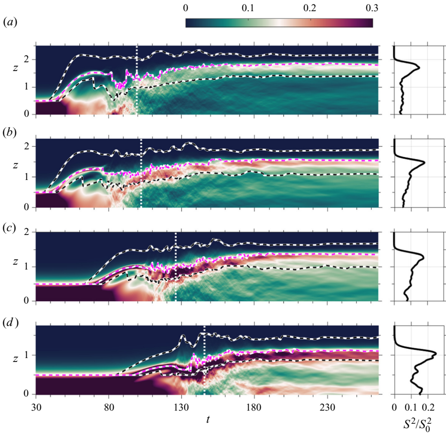
Figure 11. Similar to figure 10 but the contours show the normalized squared rate of shear ( S^2/S_0^2 ).
