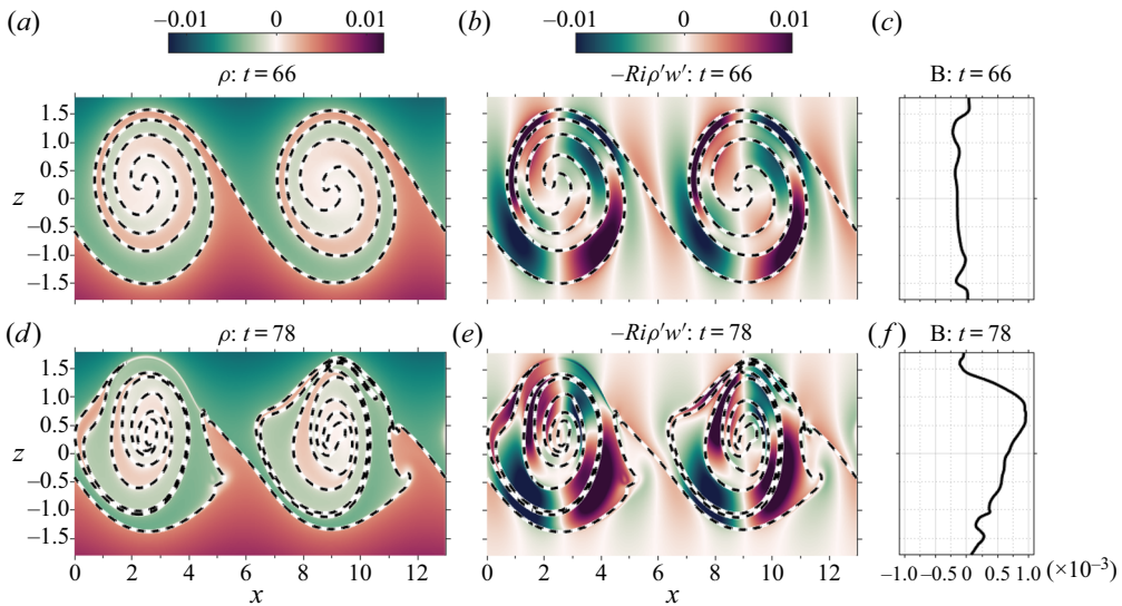
Figure 7. Cross-sectional snapshots of density ( \rho ) and buoyancy flux -Ri\rho'w' fields as well as the profiles of horizontally averaged buoyancy flux ( B ) in the Ri = 0.04 case at two times: (a–c) before the contraction at t = 66 and (d–f) during the contraction at t = 78 . The x – z planes are extracted at y = L_y/2 . Dashed lines show the isopycnal contour of \rho = 0 .
