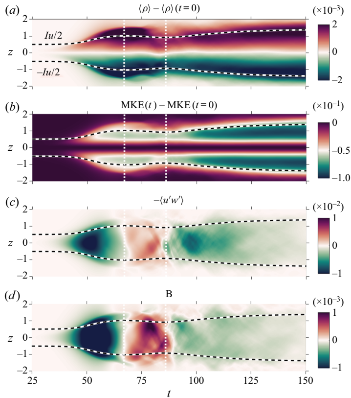
Figure 6. Evolution of the (a) density deviation from the initial profile, (b) MKE deviation from the initial profile, (c) momentum flux -\langle u'w' \rangle and (d) buoyancy flux B for the Ri = 0.04 case. Dashed lines denote the boundaries of the shear layer defined as z = \pm I_u/2 . Vertical dotted white lines mark the contraction period of the momentum thickness.
