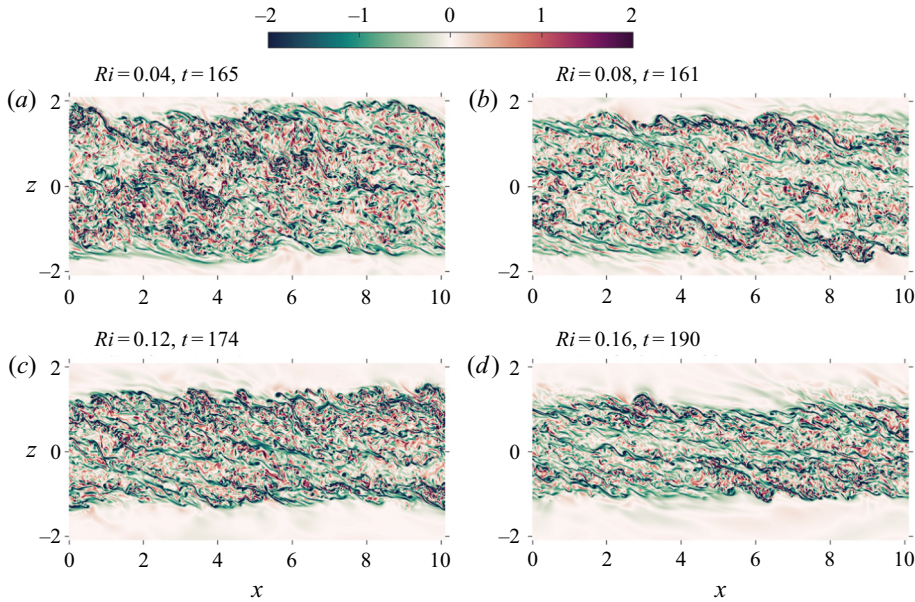
Figure 15. Cross-sectional snapshots of the spanwise vorticity ( \omega_2 ) fields for the (a) Ri = 0.04 , (b) Ri = 0.08 , (c) Ri = 0.12 and (d) Ri = 0.16 cases.
