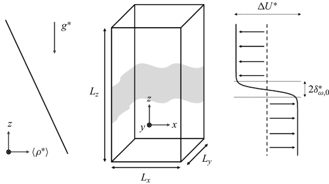
Figure 1. Sketch of the stratified shear layer with constant stratification.
