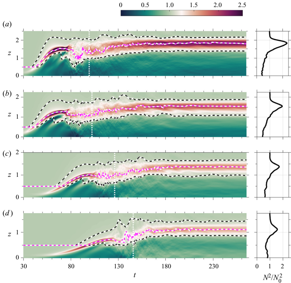
Figure 10. Evolution of the normalized squared buoyancy frequency ( N^2/N_0^2 ) shown using t - z contours for the (a) Ri = 0.04 , (b) Ri = 0.08 , (c) Ri = 0.12 and (d) Ri = 0.16 cases. The inner ( TL_i ) and outer ( TL_o ) TL boundaries are each identified using a black dashed line while the location of maximum N^2/N_0^2 inside the shear layer ( TL_m ) is shown with a magenta dashed line. Panels are given on the right for each case to illustrate vertical profiles of N^2/N_0^2 at t \approx 250 when the turbulence has subsided. The dotted white lines in all panels indicate the time of maximum dissipation rate ( t_{3d} ).
