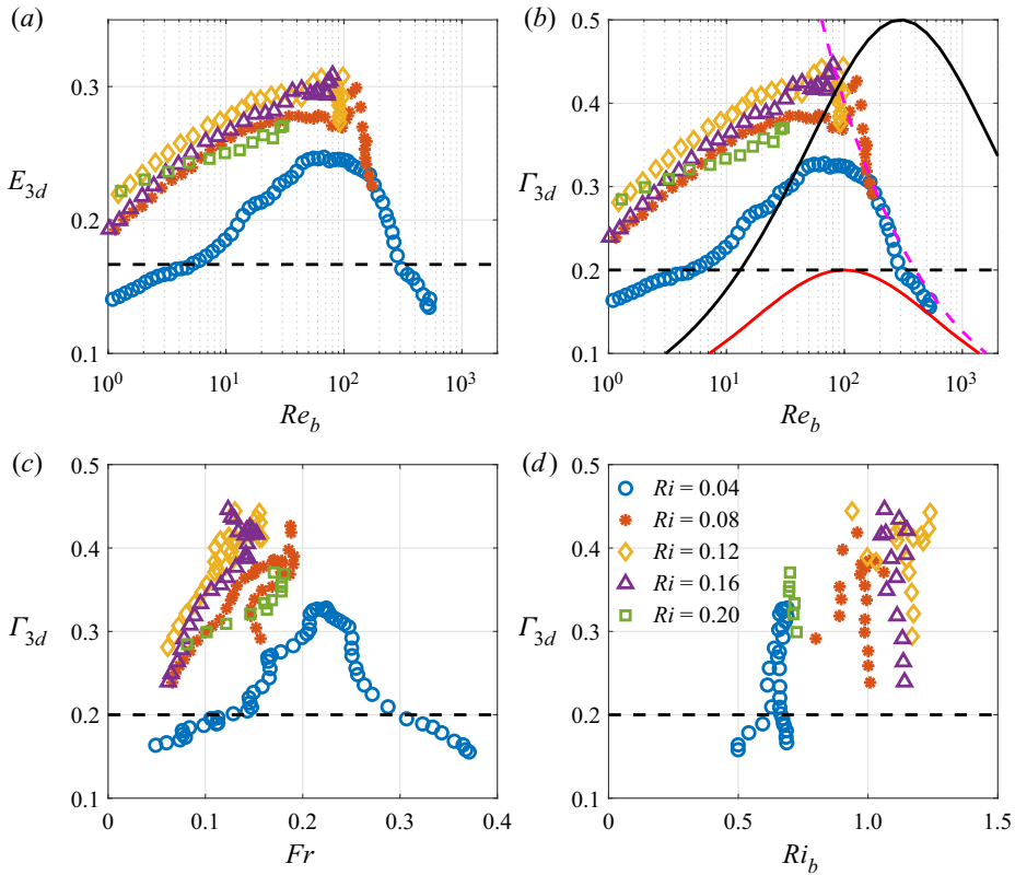
Figure 17. Effect of buoyancy Reynolds number ( Re_b ) on (a) mixing efficiency ( E_{3d} ), and (b) flux coefficient ( \Gamma_{3d} ) and the effect of (c) turbulent Froude number ( Fr ) and (d) bulk Richardson number ( Ri_b ) on the flux coefficient during the turbulent phase. The dashed black lines indicate the values of E_{3d} = 1/6 and \Gamma_{3d} = 0.2 suggested by Osborn (1980). The dashed magenta line in panel (b) indicates the parameterization, \Gamma_{3d} = 4Re_b^{-1/2} for Re_b > 10^2 in the Ri = 0.04 case. The solid black and red lines in panel (b) denote the upper and lower bounds, respectively, of the parameterization proposed by Mashayek et al. (2017b).
