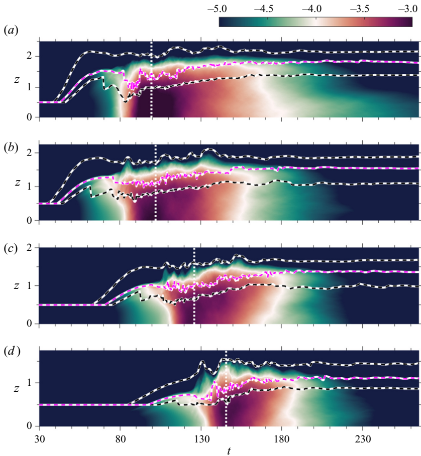
Figure 13. Similar to figure 10 but the contours show the dissipation rate ( \log_{10}(\epsilon) ).
