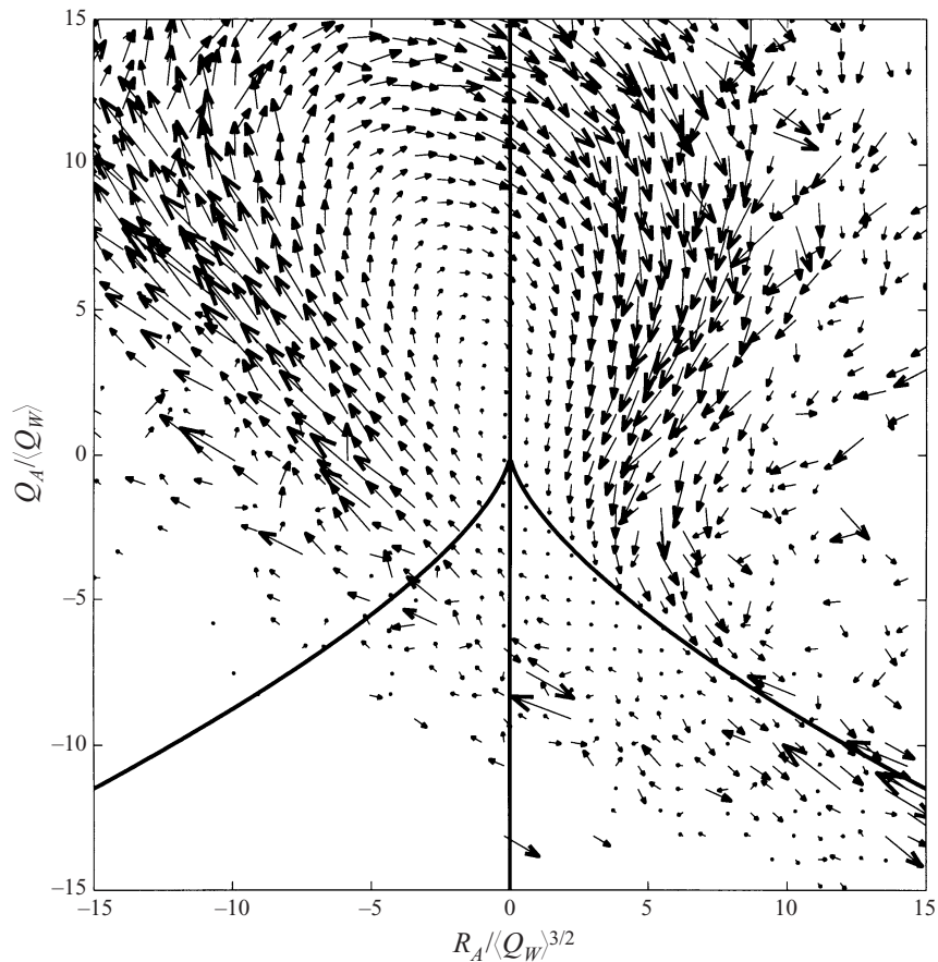
FIGURE 12. Conditional mean vectors of \hat{Q}_A and \hat{R}_A computed from data of forced isotropic turbulence at Re_\lambda = 70.9 .
