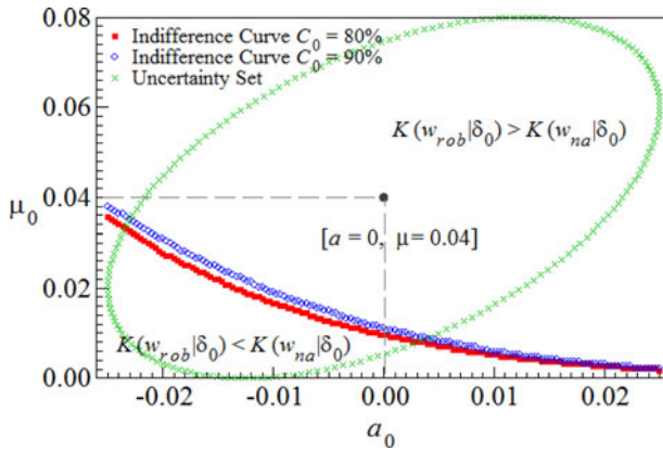
Figure 4. Loss function equivalent curves. The figure plots the indifference curve of the loss when K(w_{rob}|\delta_0) = K(w_{na}|\delta_0) . y -axis is the true value of the expected stock return \mu_0 and x -axis is the true value of the liability drift a_0 . The estimated value is \mu = 0.04 and a = 0 . The solid-dot indifference curve represents the case when C_0 = 80\% and the open-dot curve is the when C_0 = 90\% . In the region below the curve, the robust policy outperforms the naive policy, and in the region above, it is the other way around.
