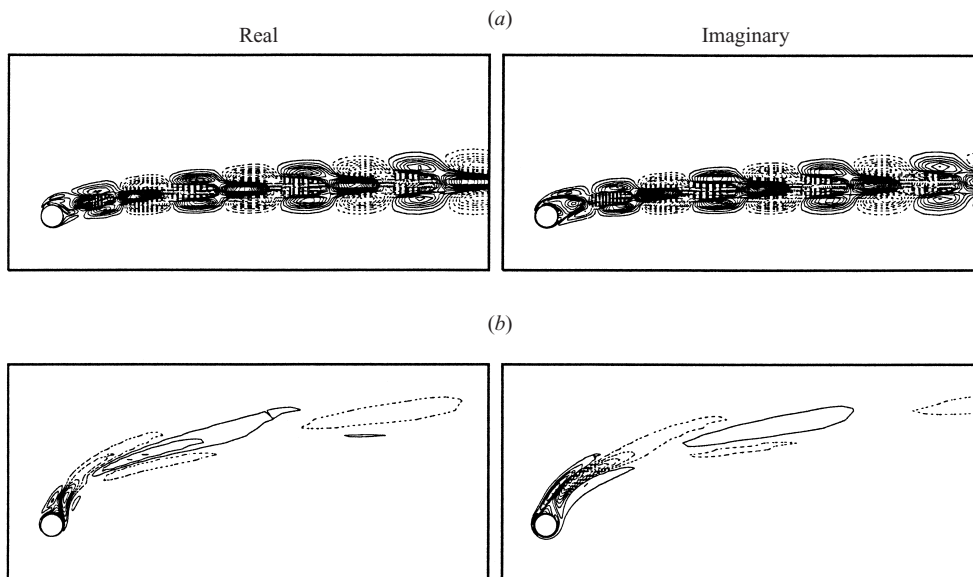
FIGURE 16. Re = 200 flow past a rotating cylinder: real and imaginary parts of the vorticity field for the most unstable mode for \alpha = 1.91 (a) and \alpha = 4.37 (b).
