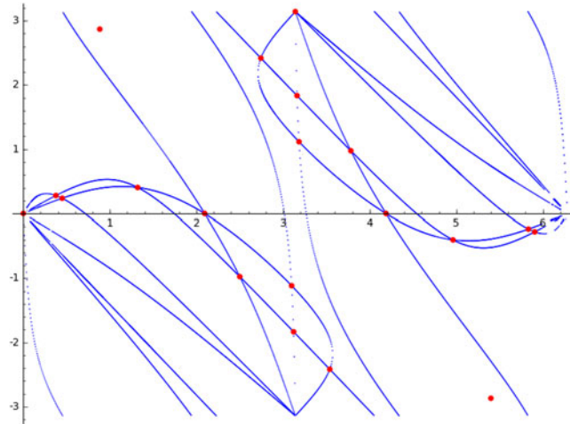
FIGURE 3. Points on the torus (axes are the arguments of x and y ). The singular points, represented by a small disc, are all intersections of one-dimensional branches, but two are isolated.
