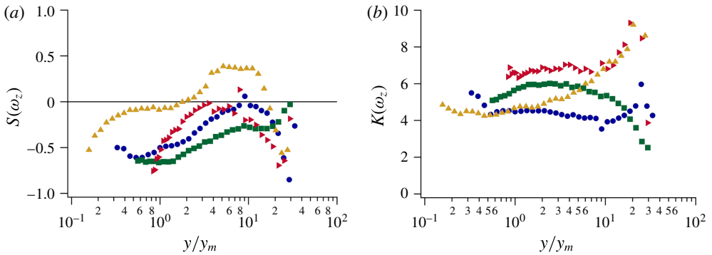
FIGURE 17. (Colour online) Higher-order central moment profiles of the spanwise vorticity fluctuations; (a) skewness, (b) kurtosis. Symbols same as in figure 6.
