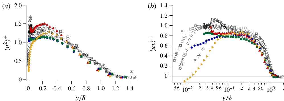
FIGURE 7. (Colour online) (a) Inner-normalized wall-normal velocity variance profiles plotted versus y/\delta ; (b) inner-normalized Reynolds shear stress profiles plotted versus y/\delta . Smooth-wall profile of DeGraaff & Eaton (2000), \delta^+ = 4580 (*); \delta^+ = 2915 , k_s^+ = 56 profile of Connelly et al. (2006) (#); other symbols same as in figure 6.
