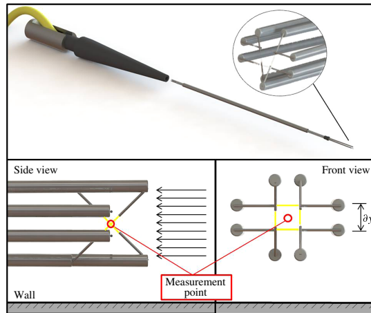
FIGURE 5. (Colour online) Four wire Foss-style \omega_z sensor used to acquire the present measurements. Note that both the unplated wire length ( 2.5 \mu\text{m} diameter) and the wire spacings are \Delta y = \Delta z = 0.5 \text{ mm} .
