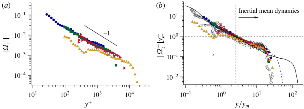
FIGURE 13. (Colour online) Normalized profiles of the mean vorticity magnitude, |\Omega_z| \simeq \partial U / \partial y ; (a) inner-normalized versus y^+ , (b) normalized using y_m and u_\tau and plotted versus y/y_m ; Hutchins et al. (2009) \delta^+ = 16\,700 , smooth (—); Schultz & Flack (2007) \delta^+ = 4760 , smooth (---); other symbols same as in figure 6. Vertical dashed line at y/y_m \simeq 2.5 .
