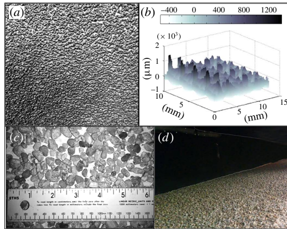
FIGURE 4. (Colour online) (a) Image of the 24-grit sandpaper roughness. (b) Surface characterization of 24-grit sandpaper roughness (courtesy of M. Schultz) as adapted from Mehdi (2012). (c) Image of the pea-gravel surface with a ruler shown for scale. (d) Pea-gravel roughness distributed along the 8 m test section.
