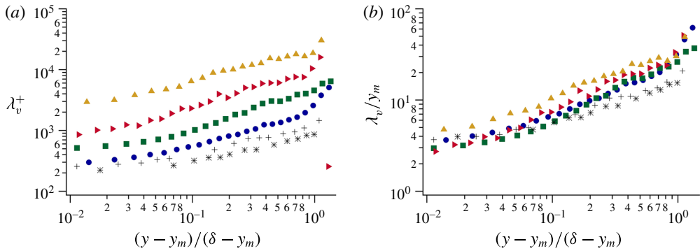
FIGURE 24. (Colour online) Inertial layer profiles of the characteristic wavelengths associated with the peaks in the premultiplied v spectra; (a) normalized by \nu/u_\tau , (b) normalized by y_m . Symbols same as in figure 14.
