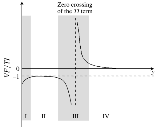
FIGURE 1. Sketch of the ratio of the ratio of terms, VF/TI , appearing in (1.1) for any given Reynolds number. Note that in rough-wall flow layer I is not present.
