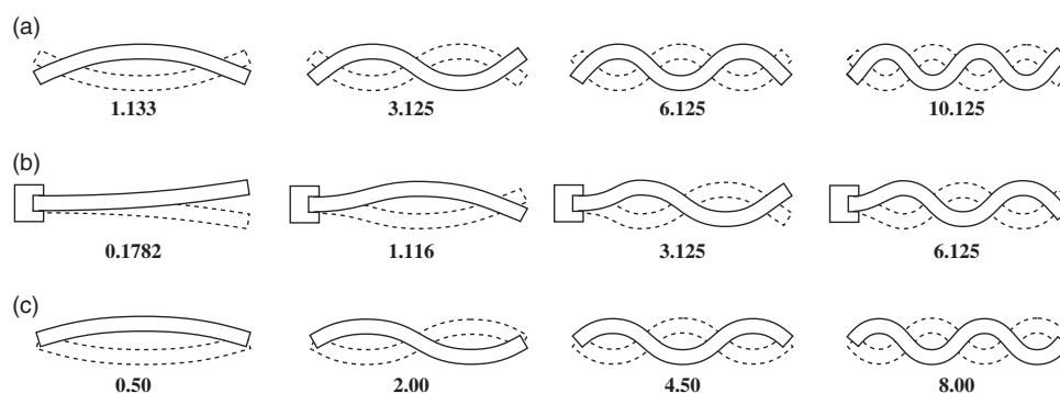
Figure 3. The resonant frequencies of a bar depends on the way the bar is mounted. Bending vibrations of (a) bar with free ends, (b) bar with one clamped end and (c) bar with two supported ends. The numbers are relative frequencies (Fletcher and Rossing 2010: 64).
