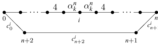
Figure 12: The doubly-truncated orthoschemes \widehat{V}_i(\alpha_k^n), 1 \leq i \leq n - 1 .
