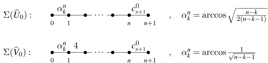
Figure 10: The graphs of \widehat{U}_0(\alpha_k^n) and \widehat{V}_0(\alpha_k^n) .
