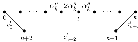
Figure 11: The doubly-truncated orthoschemes \widehat{U}_i(\alpha_k^n), 1 \leq i \leq n .
