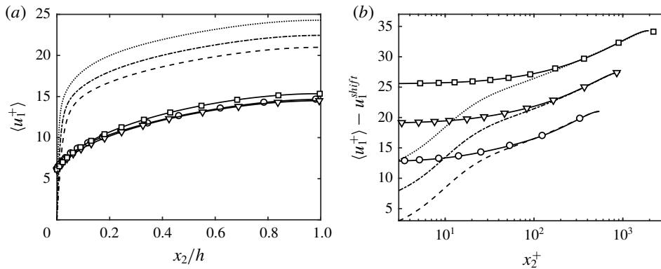
FIGURE 8. Mean streamwise velocity profiles as a function of x_2 in (a) linear scale and (b) logarithmic scale for R550 ( \circ ), R950 ( \nabla ), R2000 ( \square ), NS550 (---), NS950 (-.-.-) and NS2000 ( \cdots\cdots ). In panel (b), the velocity profiles of Robin-bounded cases are vertically shifted such that the centreline velocity coincides with their corresponding wall-bounded case. For clarity, profiles at Re_\tau \approx 950 and Re_\tau \approx 2000 are additionally shifted by 5 and 10 plus units, respectively.
