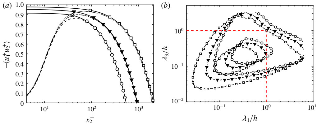
FIGURE 6. (Colour online) (a) Mean tangential Reynolds stress as a function of the wall-normal (or boundary-normal) coordinate for R550 ( \circ ), R950 ( \blacktriangledown ), R2000 ( \square ), NS550 (---), NS950 (-·-·-) and NS2000 (·····). (b) Premultiplied boundary-normal two-dimensional velocity spectra for Robin-bounded channels at x_2/h = 0 . Contours are 0.1 and 0.6 of the maximum. The red dashed lines are \lambda_1/h = 1 and \lambda_3/h = 1 . Symbols are as in panel (a).
