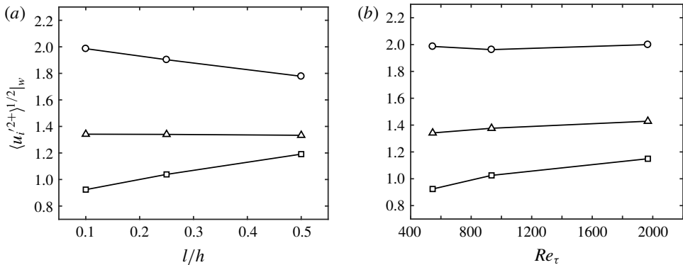
FIGURE 17. Streamwise (○), wall-normal (□) and spanwise (△) r.m.s. fluctuating velocities at x_2/h = 0 for Robin-bounded cases as a function of (a) slip length and (b) friction Reynolds number.
