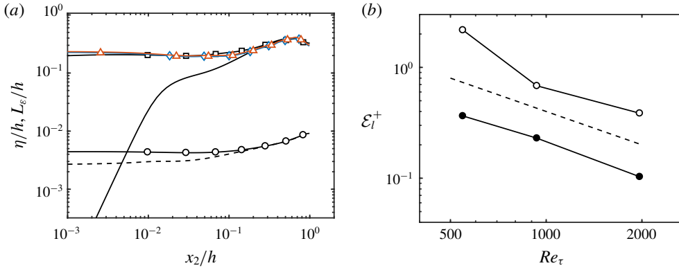
FIGURE 12. (Colour online) (a) Kolmogorov length scale \eta for NS550 (---) and R550 (○), and integral length scale L_\epsilon for NS550 (—), R550 (□), R950 (◇) and R2000 (△). (b) \mathcal{E}_l^+ as a function of Re_\tau . Closed and open symbols are for wall-bounded and Robin-bounded cases, respectively. The dashed line is \mathcal{E}_l^+ \sim Re_\tau^{-1} .
